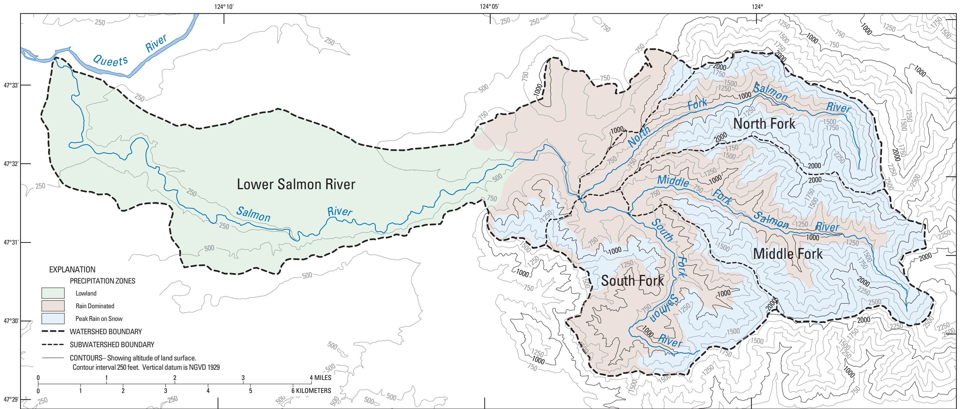
Figure 5. Precipitation zones in the Salmon River watershed, delineated by the Washington Department of Natural Resources.
