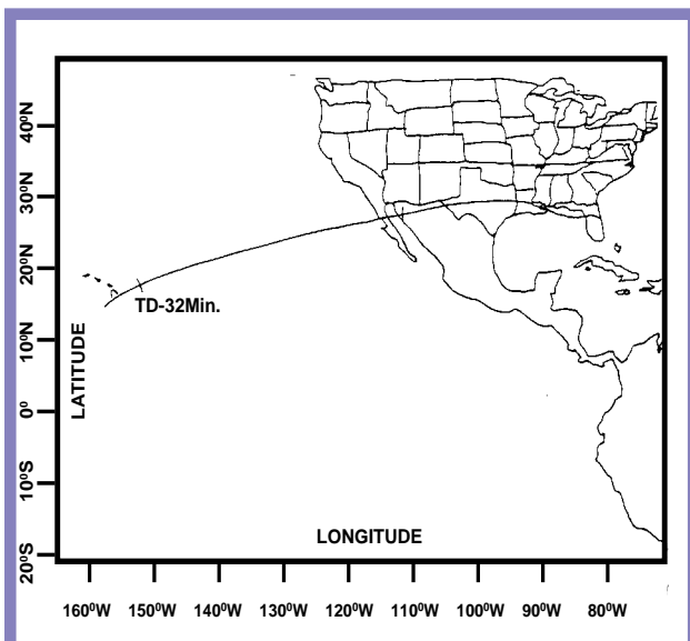
This map shows the ground track of a typical low-inclination orbit.
