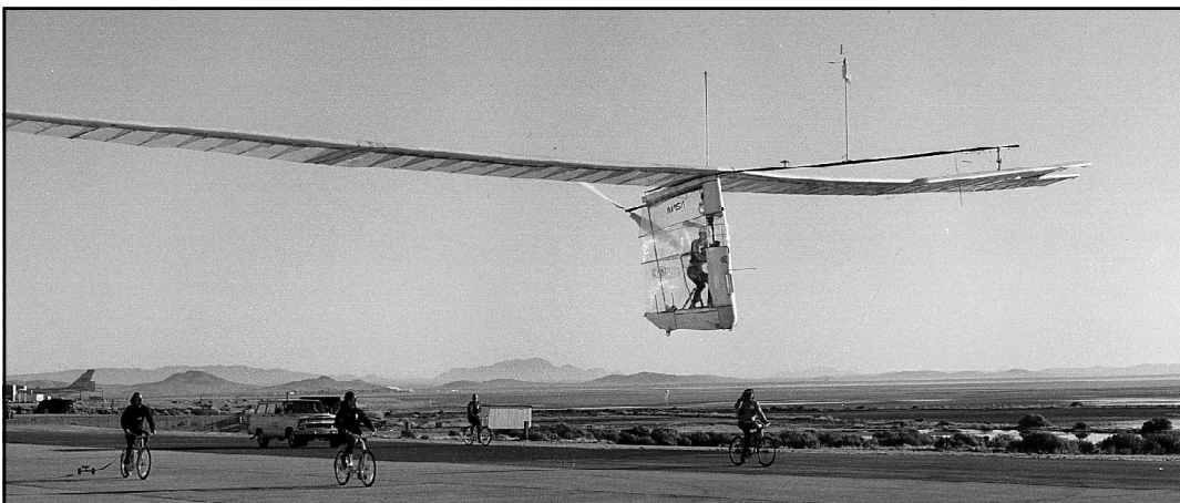
During the early part of 1980, in a joint project with NASA's Langley Research Center and AeroVironment, NASA's Dryden Flight Research Center gathered data on a Gossamer Albatross in which the light-weight aircraft flew under three conditions: using human power, using a small electric motor, and in a towed condition with the propeller removed. NASA photo ECN 12558
