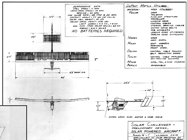
Artist's conception of Solar Challenger (left). Preliminary design of Solar Challenger (above). Photos courtesy of Du Pont Co.
