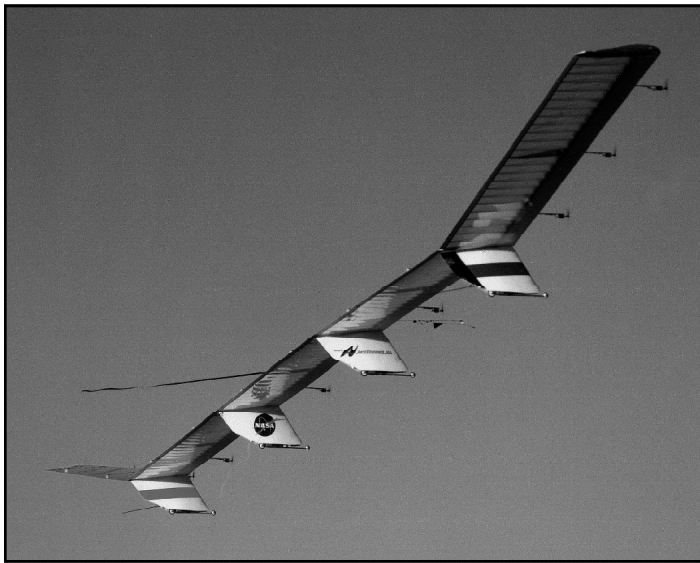
One quarter-scale model of AeroVironment's Centurion ultra-high-altitude flying wing, flown as a low-cost, low-risk proof-of-concept vehicle before going ahead with the full-scale prototype. NASA photo EC97 43965-4
