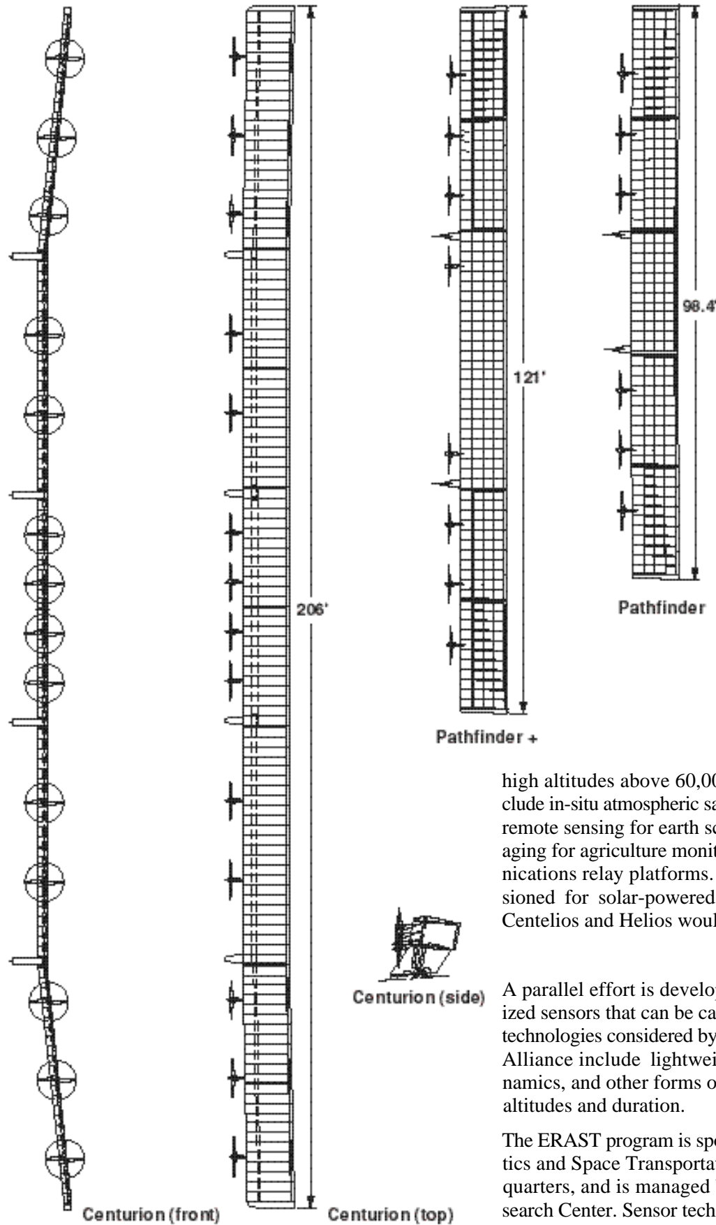
Three-view drawing of Centurion with top views of Pathfinder and Pathfinder-Plus for comparison.
