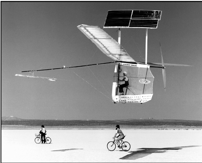
Gossamer Penguin in flight above Rogers Dry Lakebed at Edwards, Calif., showing the solar panel perpendicular to the wing and facing the sun. NASA photo ECN 13413
