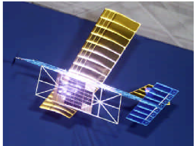
With a laser beam centered on its panel of photovoltaic cells, a model makes the first flight of an aircraft powered by a laser beam inside a building at NASA Marshall.
