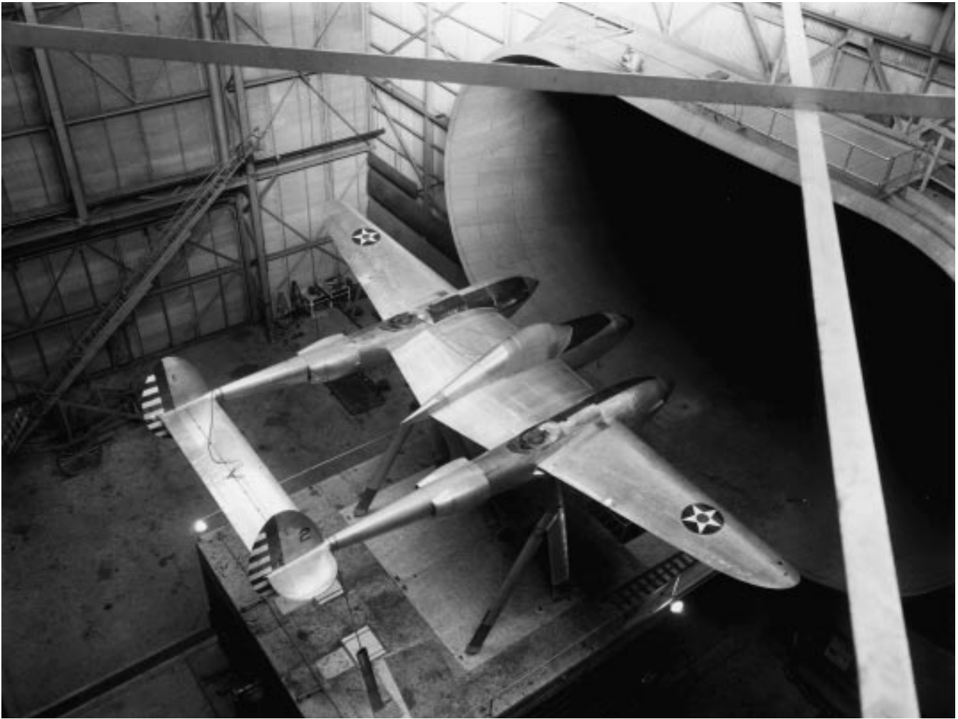
A Lockheed YP-38 Lightning (the second prototype of the Lightning series) undergoes drag clean-up in the NACA Langley 30 x 60-ft. Full-Scale Tunnel.
