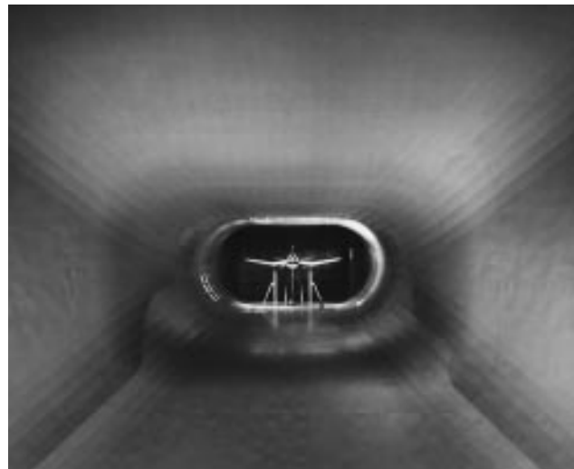
This Douglas XSBD-2 model was the first aircraft to be tested in the NACA Ames 40 x 80-ft. Wind Tunnel, the largest wind tunnel in the world at the time. Drag reduction studies were performed on the airplane.
