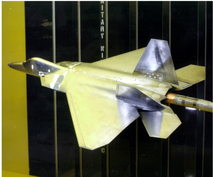
F-22 model mounted for supersonic test in the Langley Unitary Tunnel.
