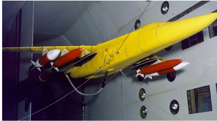
FB-111 flutter model illustrating the wide scope of external stores that were tested in the program.
