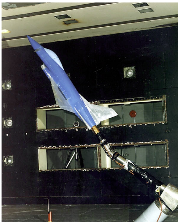
X-31 with F-16 canopy during tests in the Langley 14- by 22-Foot Low-Speed Tunnel.
