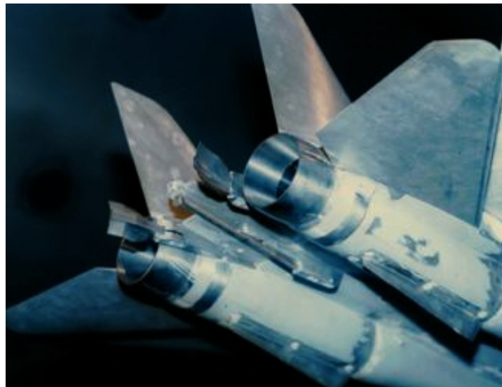
F-14 model equipped with deflectable yaw vanes in the Langley 16-Foot Transonic Tunnel.
