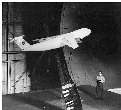
Powered C-5 model mounted in the Langley Full-Scale Tunnel for externally blown flap assessments with the double-slotted flap configuration.
