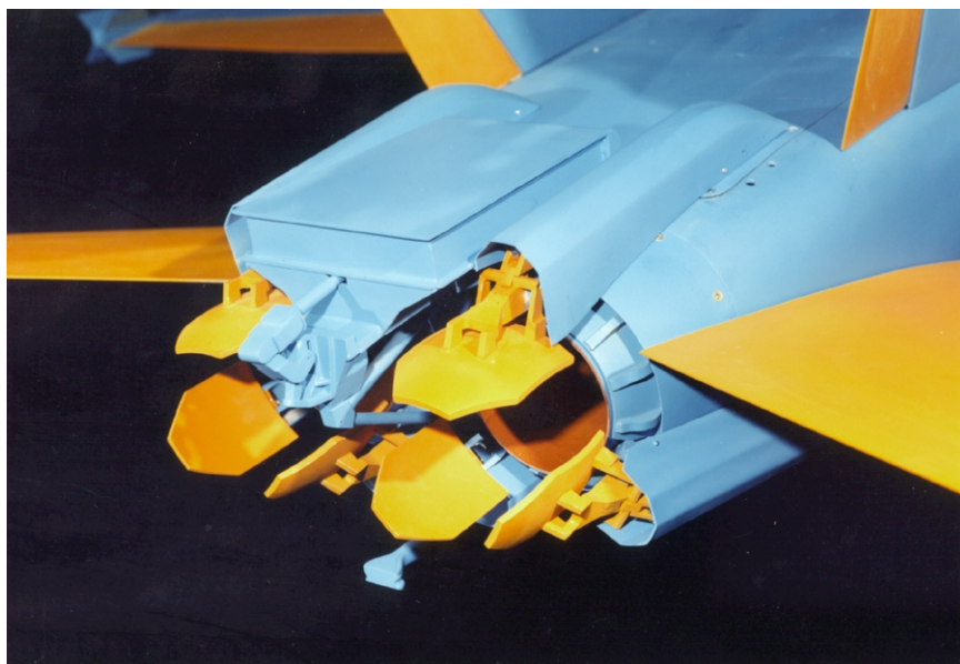
Thrust-vectoring vane installation on the F-18 HARV free-flight model with rectangular box above the vanes representing the container for the spin parachute.
