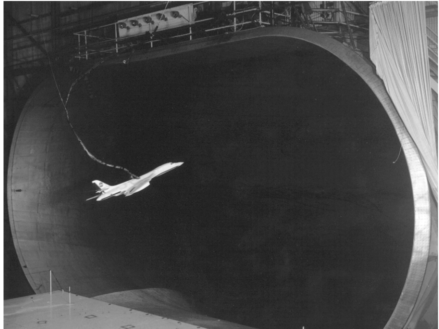
B-1A model in free-flight tests in the Langley Full-Scale Tunnel in 1972.
