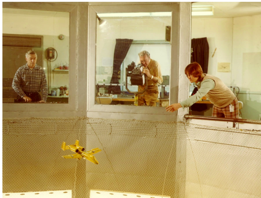
Spin tunnel tests of the A-10 configuration.
