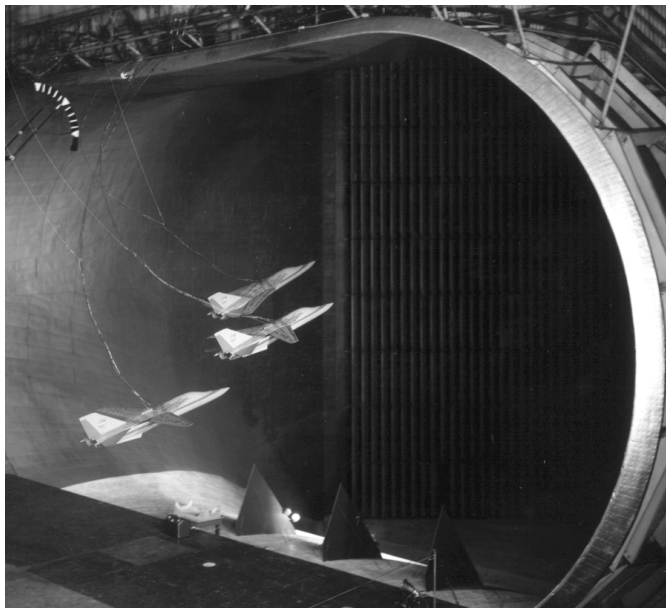
Time-lapse photograph of the F-111A free-flight model at several wings sweep angles during tests in the Langley Full-Scale Tunnel.
