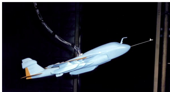
The modified EA-6B model in flight in the Full-Scale Tunnel.
