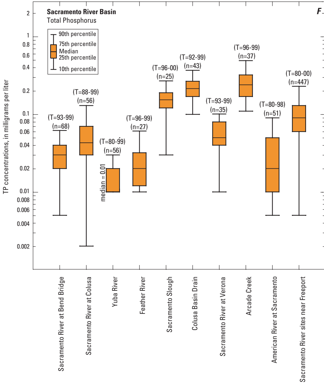
Figure 9F. Constituent concentrations in the Sacramento River Basin, California: available total phosphorus (TP) data for all the sites in the basin.
