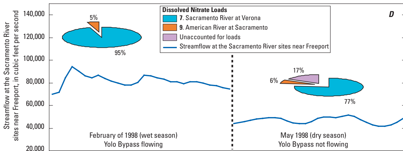
Figure 14D. Percentage of dissolved nitrate loads and hydrograph for water year 1998 for the Sacramento River sites near Freeport, California, during February 1998 for the wet season and May 1998 for the dry season.
