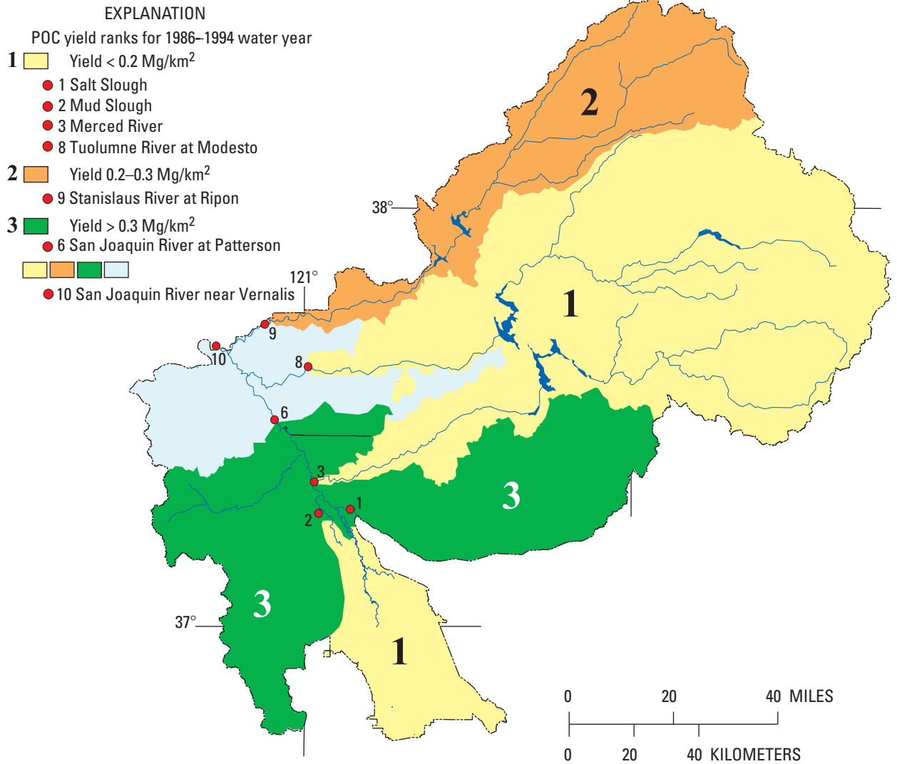
Figure 21B. Particulate organic carbon (POC) yields in the San Joaquin River Basin, California.
