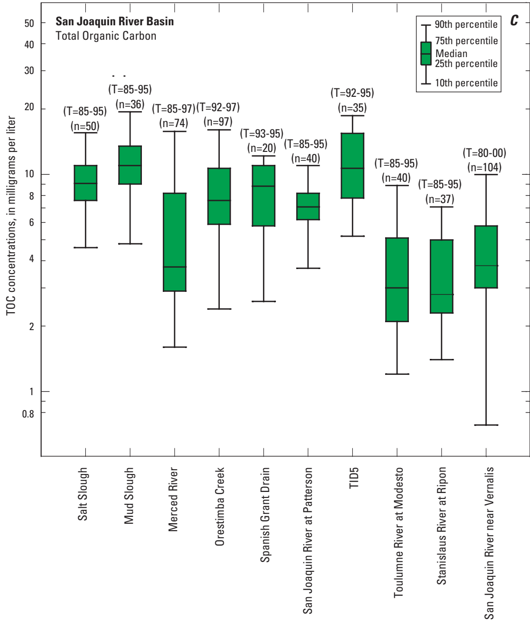
Figure 10C. Constituent concentrations in the San Joaquin River Basin, California: available total organic carbon (TOC) data for all the sites in the basin.
