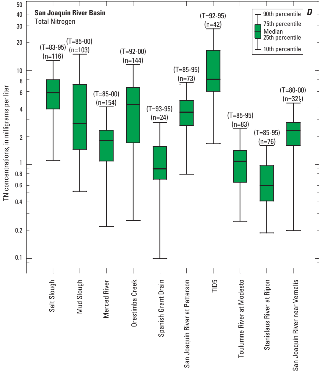
Figure 10D. Constituent concentrations in the San Joaquin River Basin, California: available total nitrogen (TN) data for all the sites in the basin.
