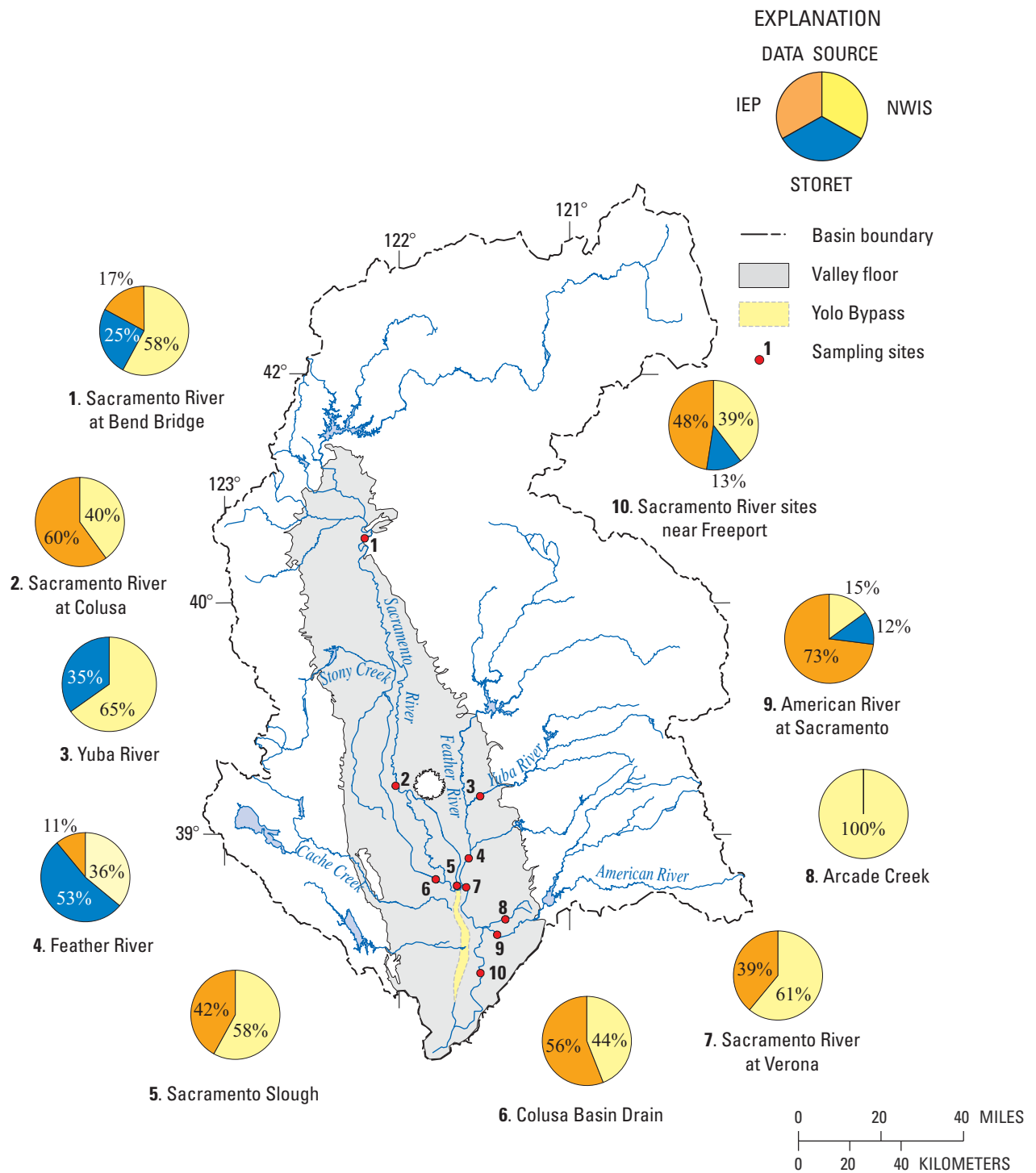
Figure 5. Percentage of data obtained for each site in the Sacramento River Basin, California, from three database sources.
