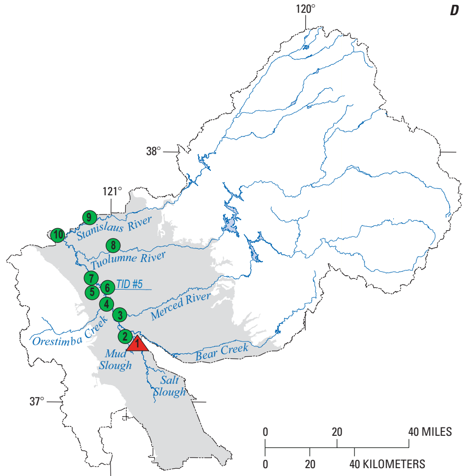
Figure 12D. Total nitrogen trends for the San Joaquin River Basin, California.
