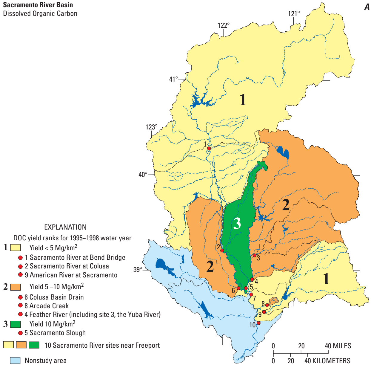
Figure 20A. Dissolved organic carbon (DOC) yields during water years 1995–1998 in the Sacramento River Basin, California.
