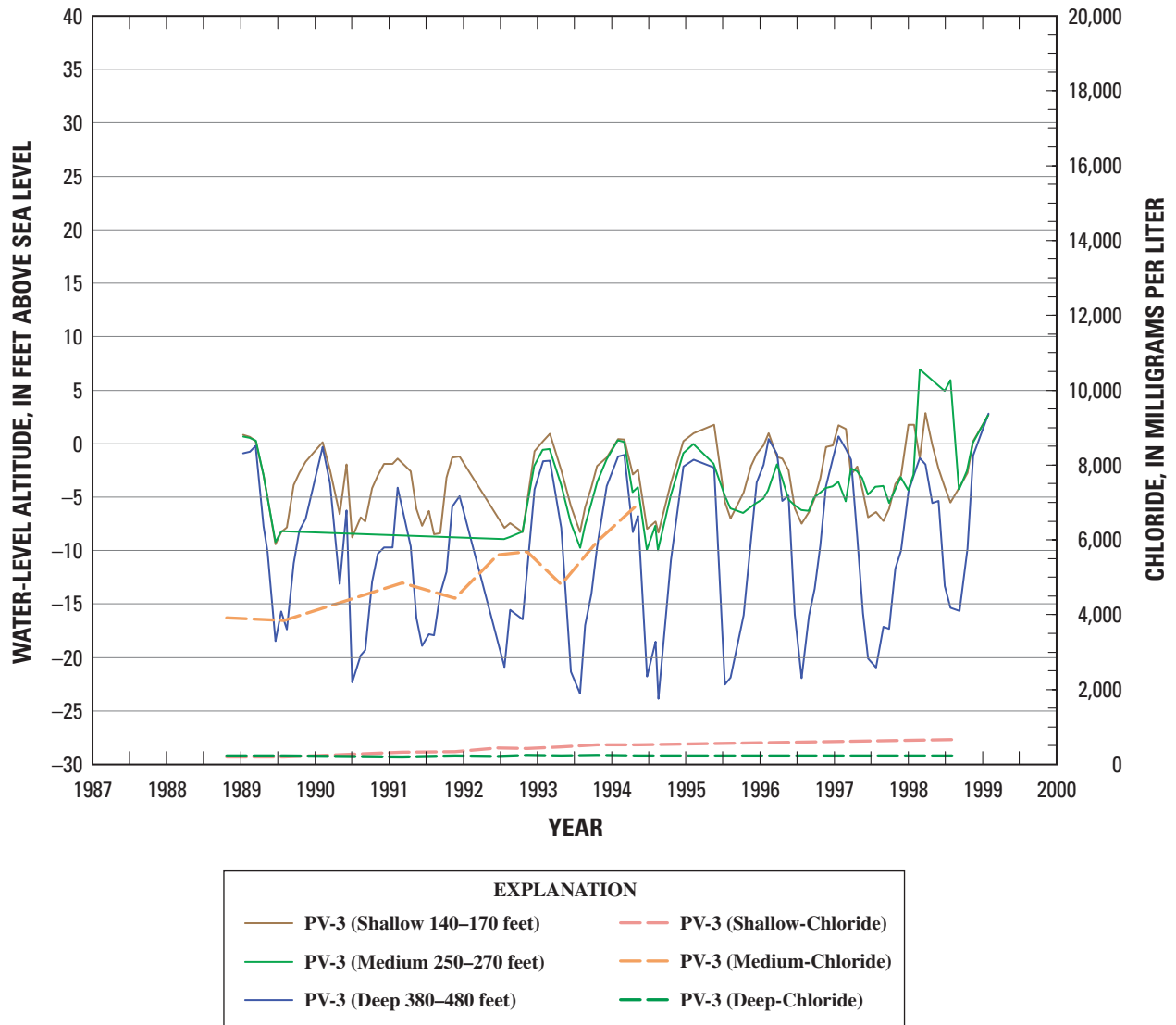
Figure 9. The PV-3 multiple-well monitoring site in the Pajaro River Mouth subarea of the Pajaro Valley, Santa Cruz County, California.
