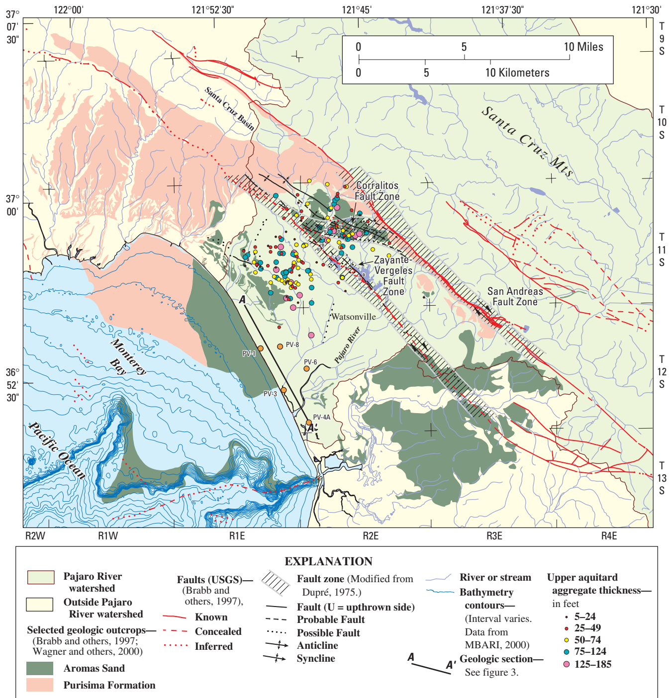
Figure 2. Geology, selected wells used to estimate aquifer thicknesses, geologic outcrops, and sites for geophysical logging in the Pajaro Valley, Santa Cruz and Monterey Counties, California.
