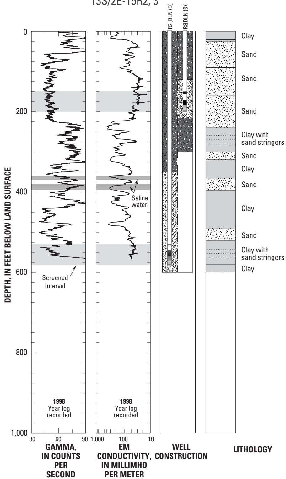
Figure A1.11. Geophysical logs and well construction for selected monitoring wells and test holes in the Pajaro Valley, Santa Cruz County, California.
