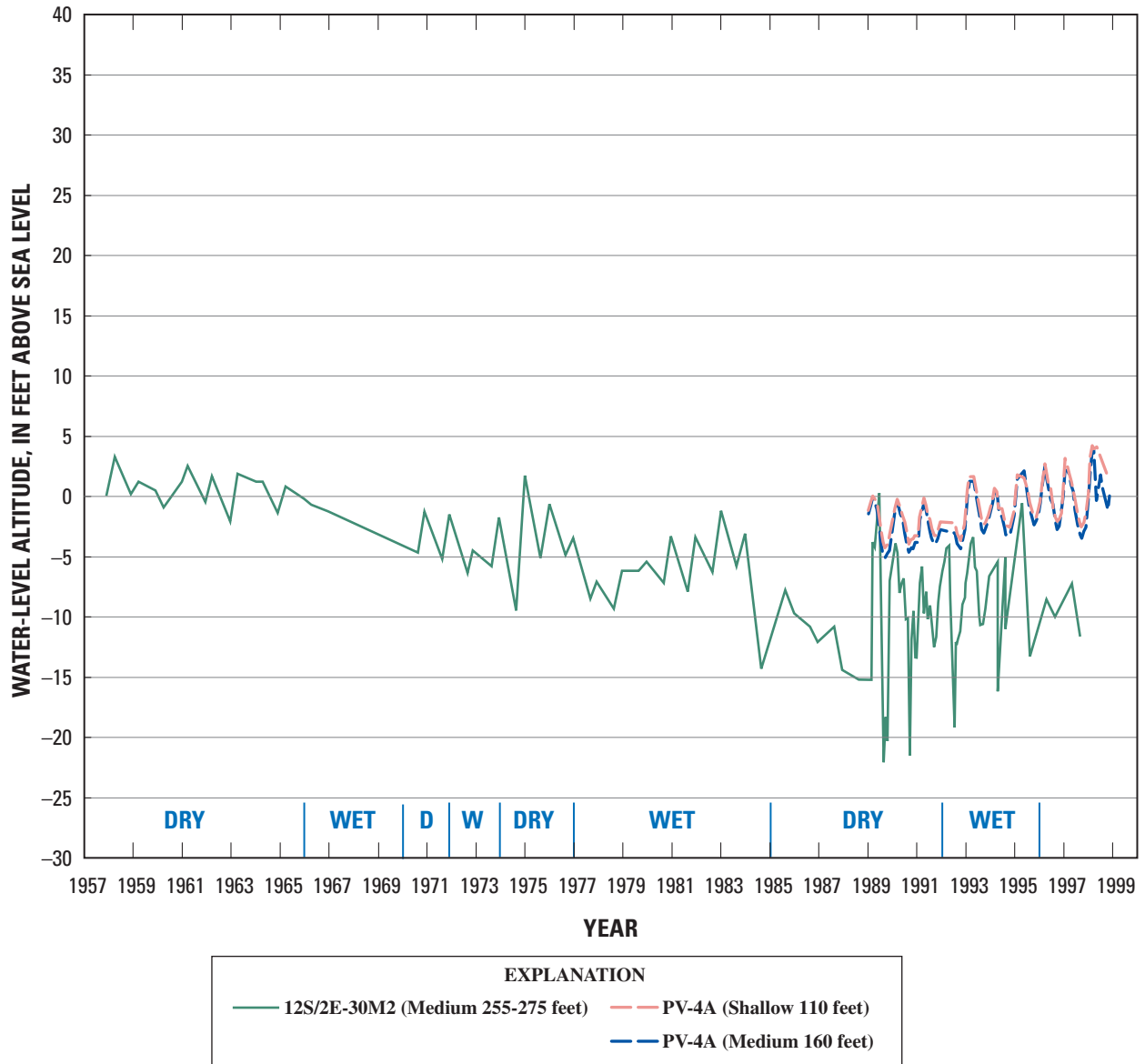
Figure 17. Multiple-well PV-4 and well 12S/2E-30M2 in the Springfield subarea of the Pajaro Valley, Monterey County, California.
