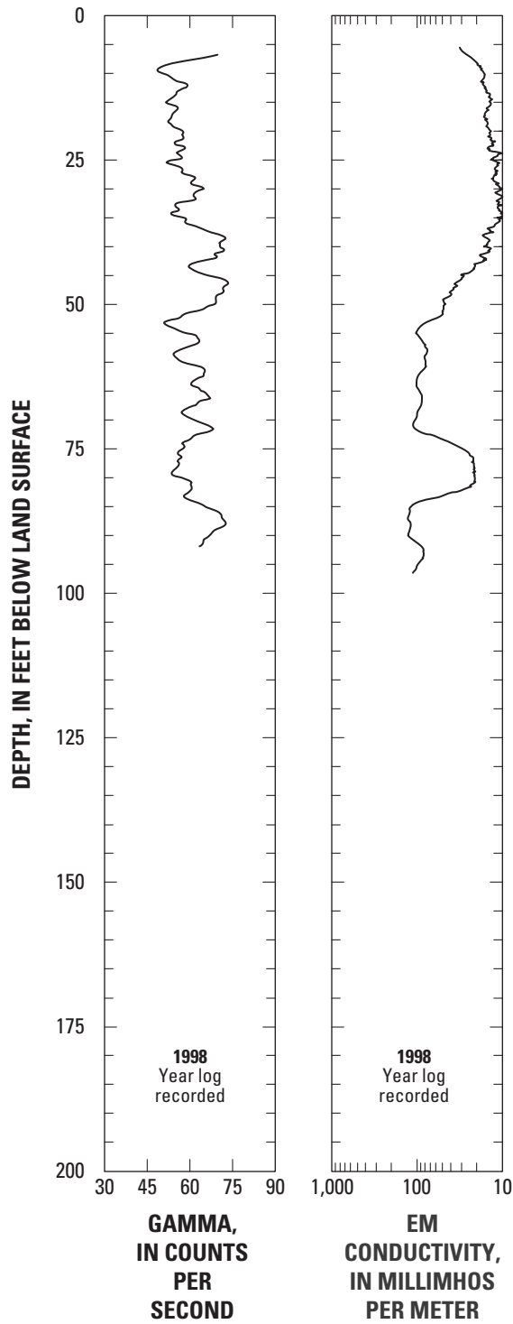
Figure A1.9. Geophysical logs and well construction for selected monitoring wells and test holes in the Pajaro Valley, Santa Cruz County, California.
