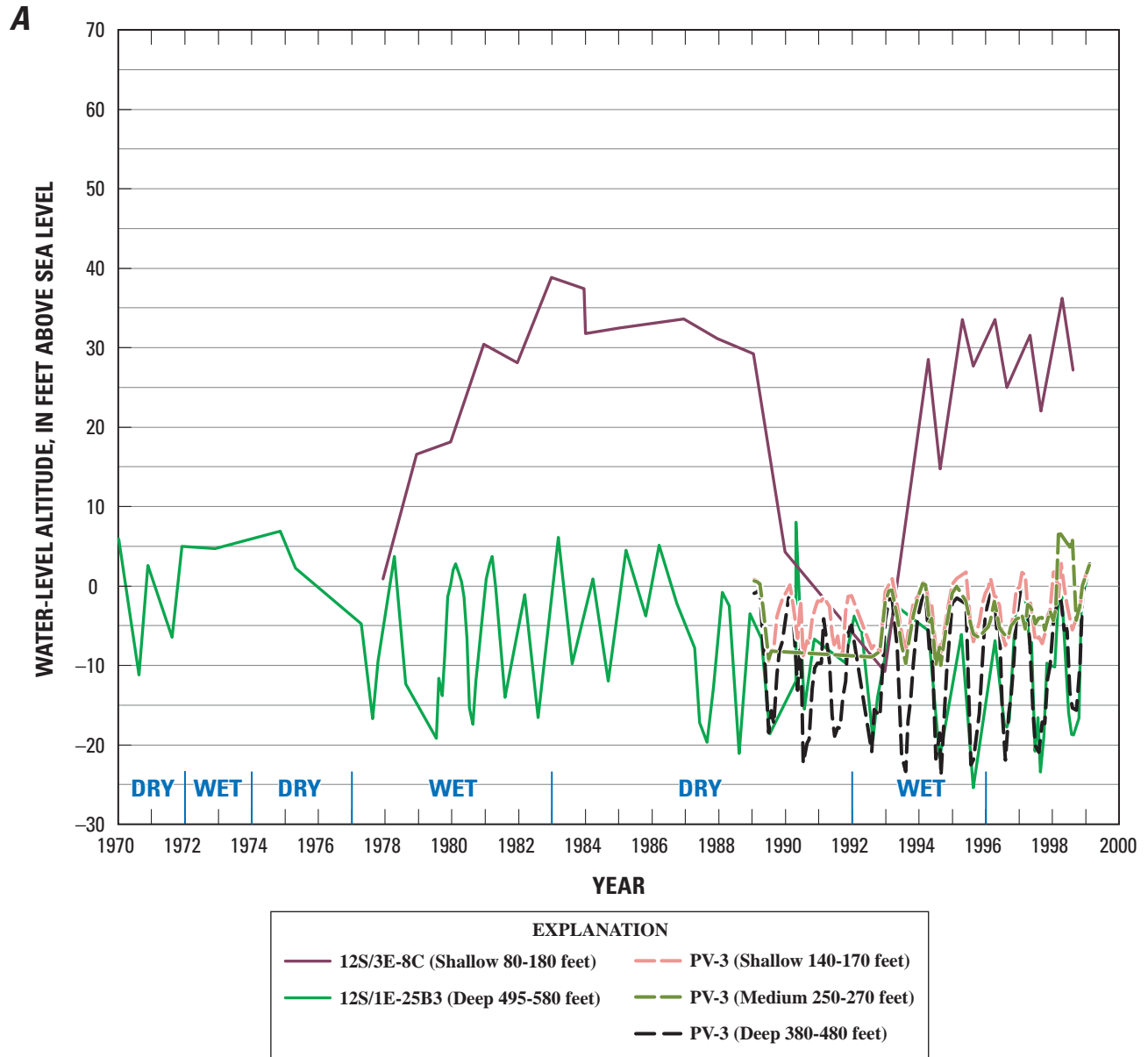
Figure 16. Multiple-well PV-3 and deep well 12S/1E-25B3 in the Pajaro River Mouth subarea and wells 12S/3E-8C and 12S/3E-7J2 in the Pajaro subarea of the Pajaro Valley, Santa Cruz County, California.
