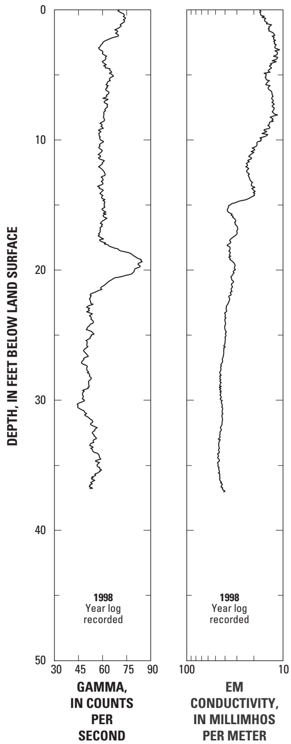
Figure A1.10. Geophysical logs and well construction for selected monitoring wells and test holes in the Pajaro Valley, Santa Cruz County, California.
