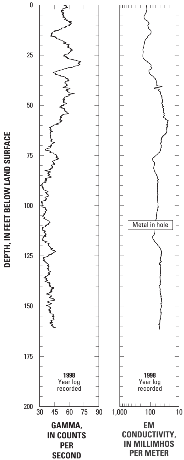
Figure A1.8. Geophysical logs and well construction for selected monitoring wells and test holes in the Pajaro Valley, Santa Cruz County, California.
