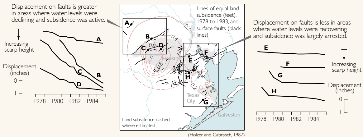
Vertical displacements at eight selected fault-monitoring sites in the Houston area show a pattern related to water-level declines and land subsidence.
