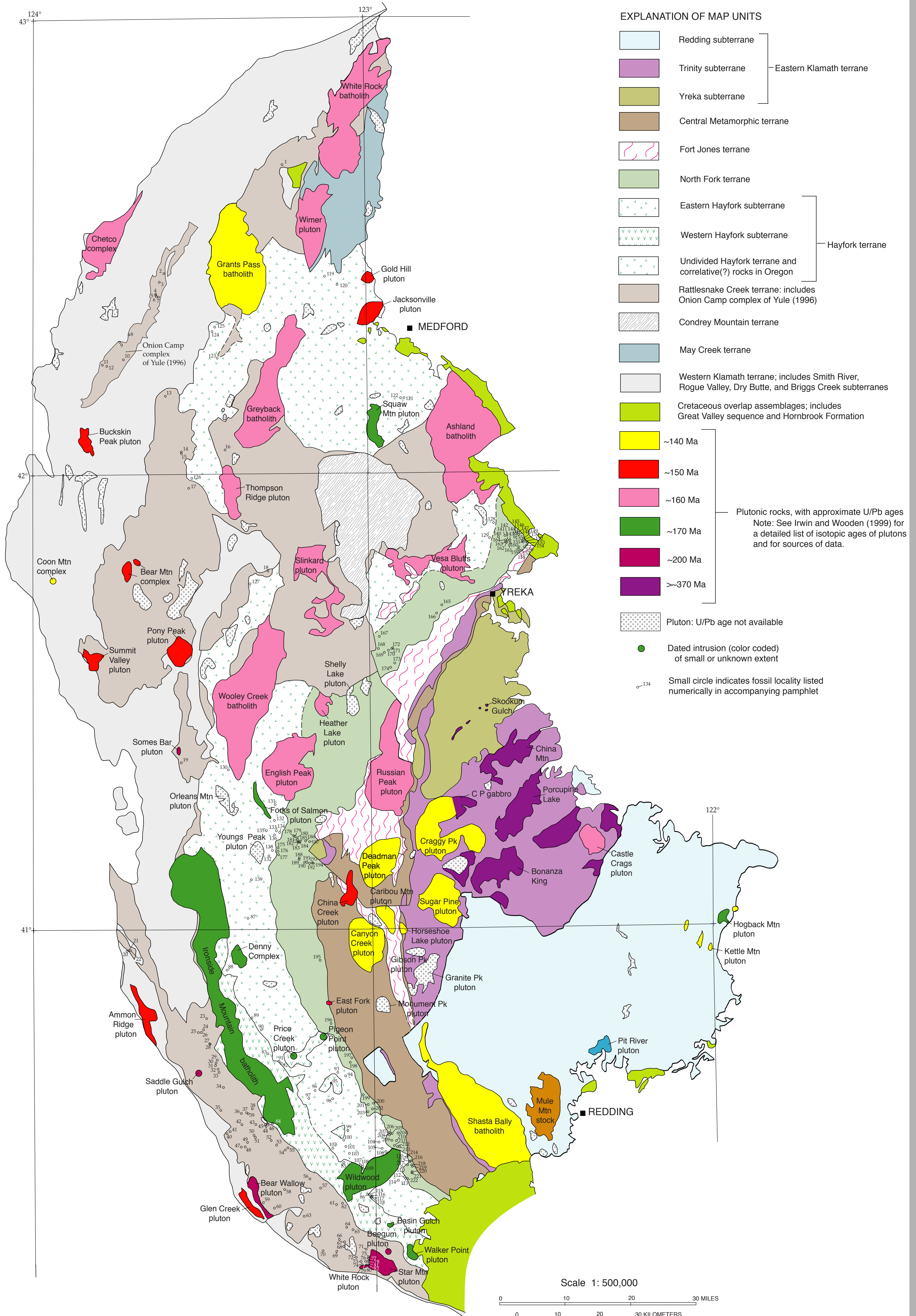
Map showing fossil localities of the North Fork, Eastern and Western Hayfork, and Rattlesnake Creek terranes of the Klamath Mountains, California and Oregon
