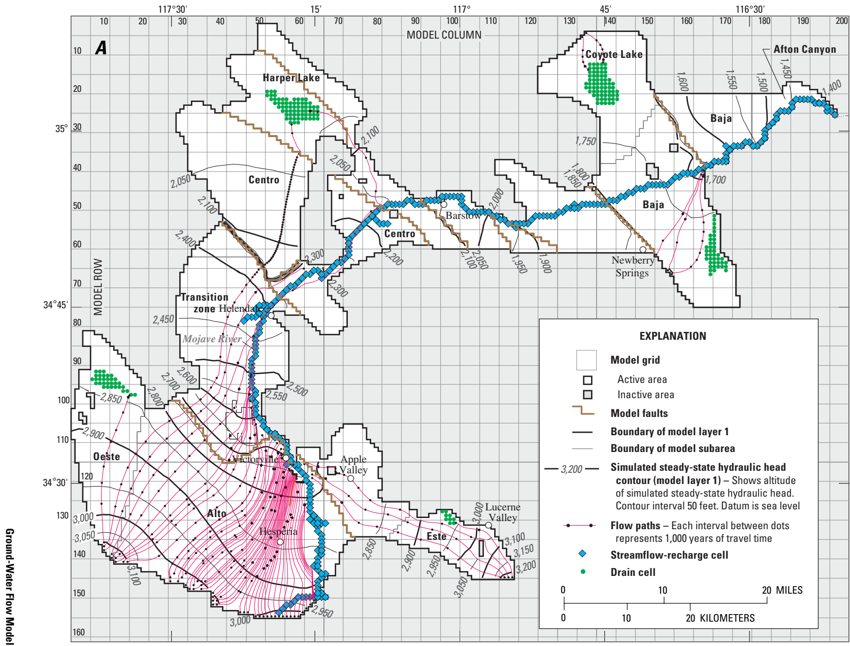
Figure 35. (A) Simulated flow paths of selected particles for steady-state (1930) conditions initially placed at mountain-front recharge cells, and (B) location of streamflow recharge cells of the ground-water flow model of the Mojave River ground-water basin, southern California.
