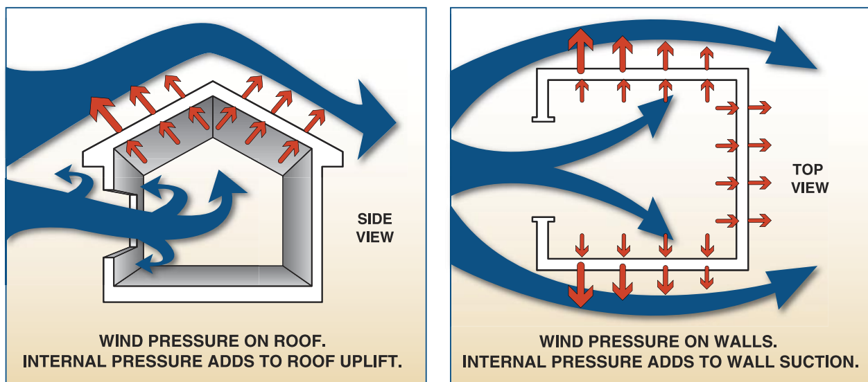
Figure II.1 Effect of extreme winds on building roof and walls
