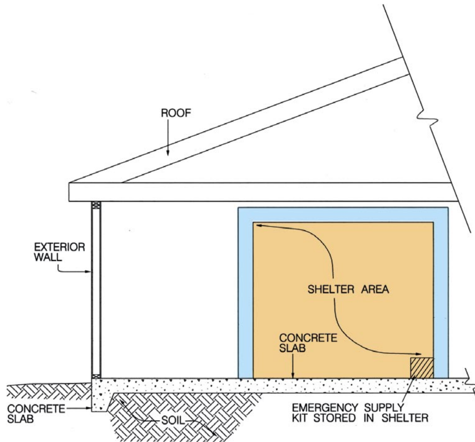
Figure II.3 Cross-section: typical slab-on- grade foundation, with shelter
