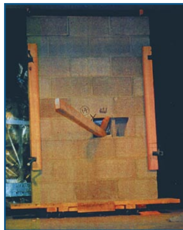
2" x 4" wood stud launched at 100 mph pierces unreinforced masonry wall, WERC, Texas Tech University
