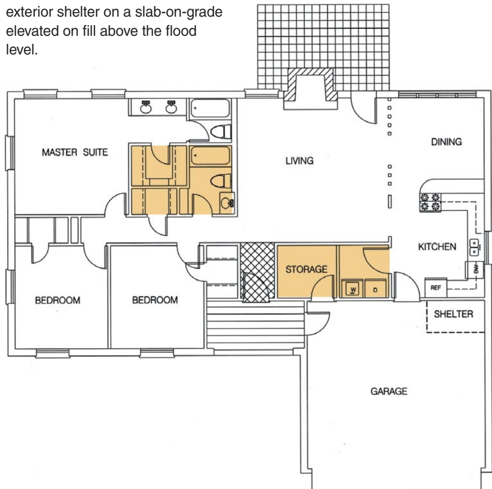
Figure II.6 Floor plan 2: house on a slab-on-grade or crawlspace foundation
