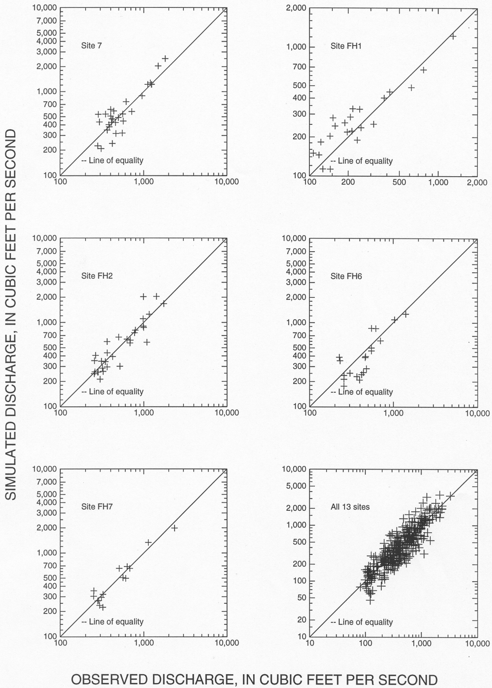
Figure 3. Comparison of observed and simulated peak discharges at selected sites and all sites combined for storms used in calibrations of the Rainfall-Runoff Model (RRM) for urban watersheds in Jefferson County, Kentucky.
