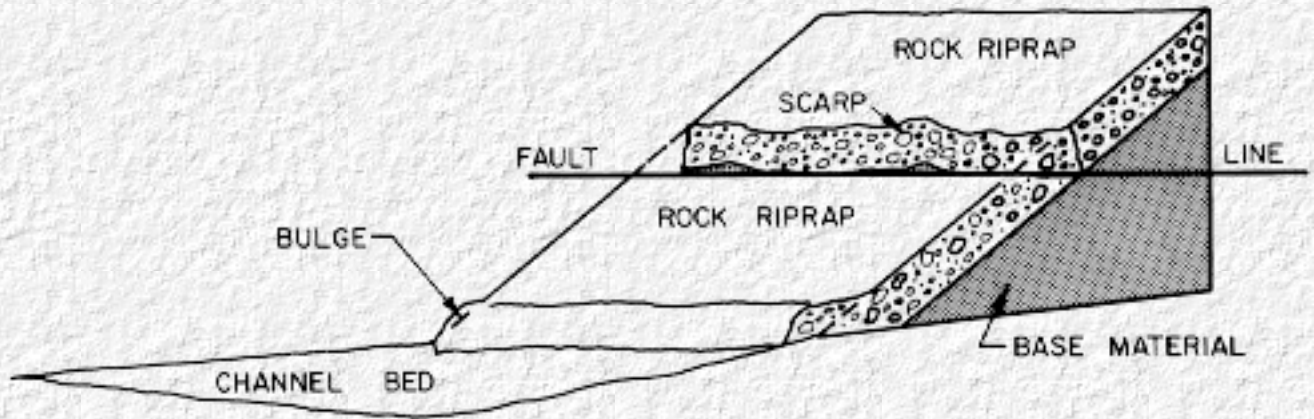
Figure 2. Translational Slide Failure (Modified from Blodgett (6))
