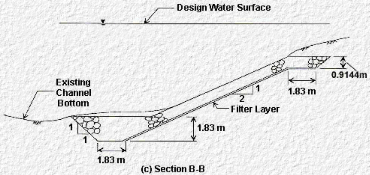
Figure 32. Toe and Flank Details; Example 2
