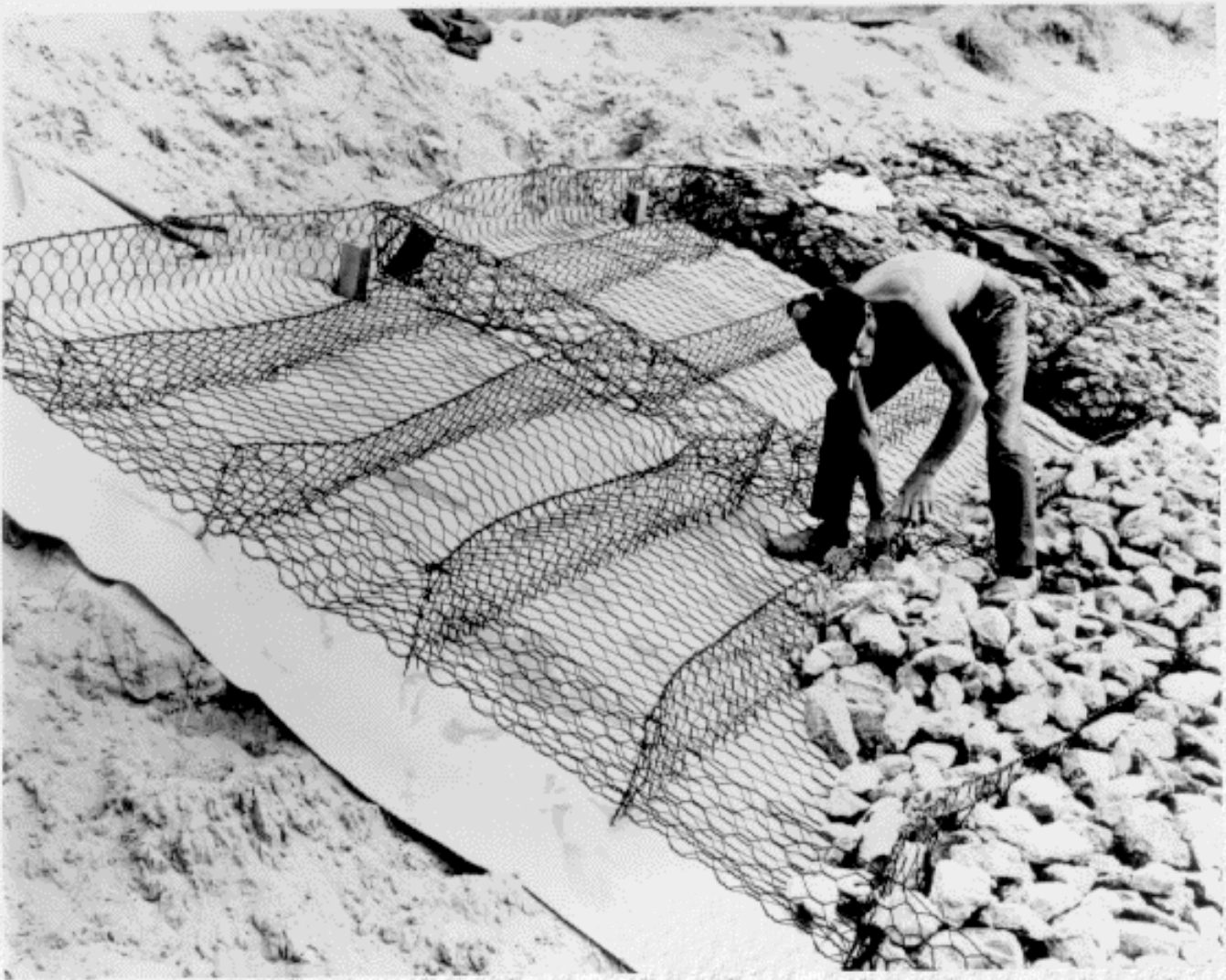
Figure 45. Rock and Wire Revetment Mattress Installation (courtesy, Maccaferri Gabions, Inc.)
