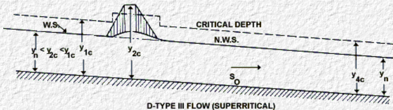
Figure 18. Typical Water Surface Profiles Through Bridge Constrictions for Various Types as Indicated (Modified from Bradley (40))
