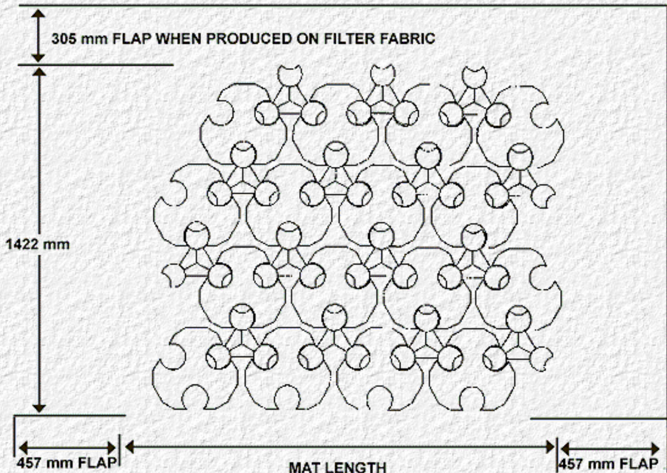
Figure 55. Tri-lock Revetment (see reference section A-A, Figure 39 )
