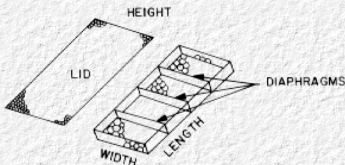
Figure 43. Mattress Configuration
