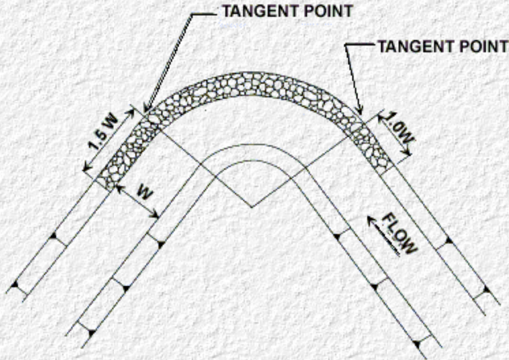
Figure 15. Longitudinal Extent of Revetment Protection
