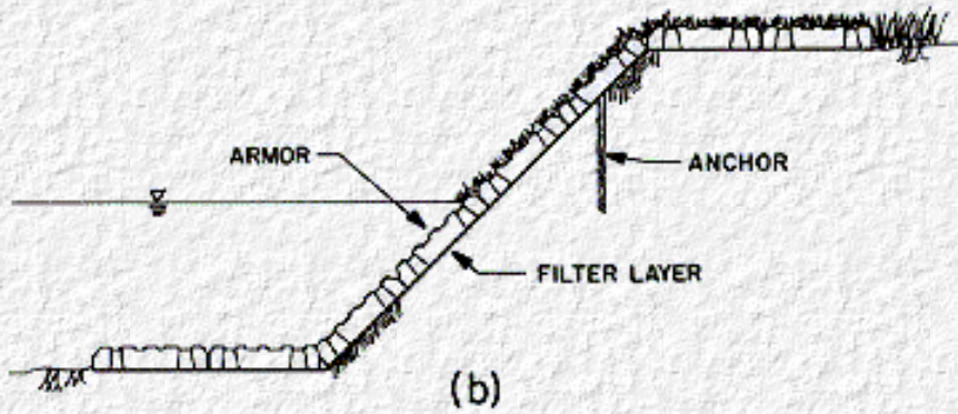
Figure 51. Monoslab Revetment (a) Block Detail and (b) Revetment Detail
