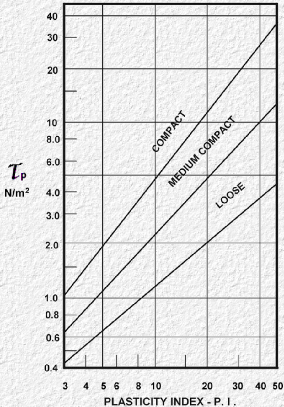
Chart 2. Permissible Shear Stress for Cohesive Soils (after 16)
