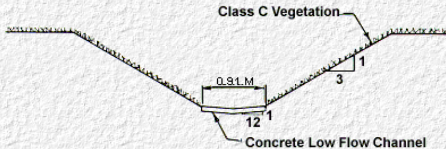
Figure 26. Compound Lining Example
