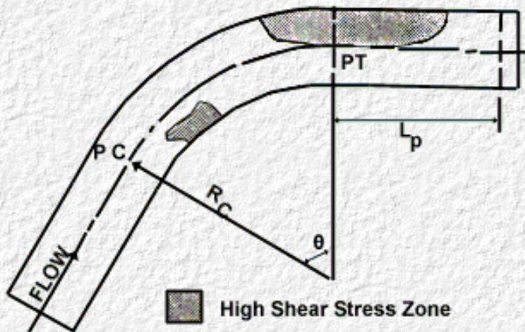
Figure 19. Shear Stress Distribution in a Channel Bend (after 11)
