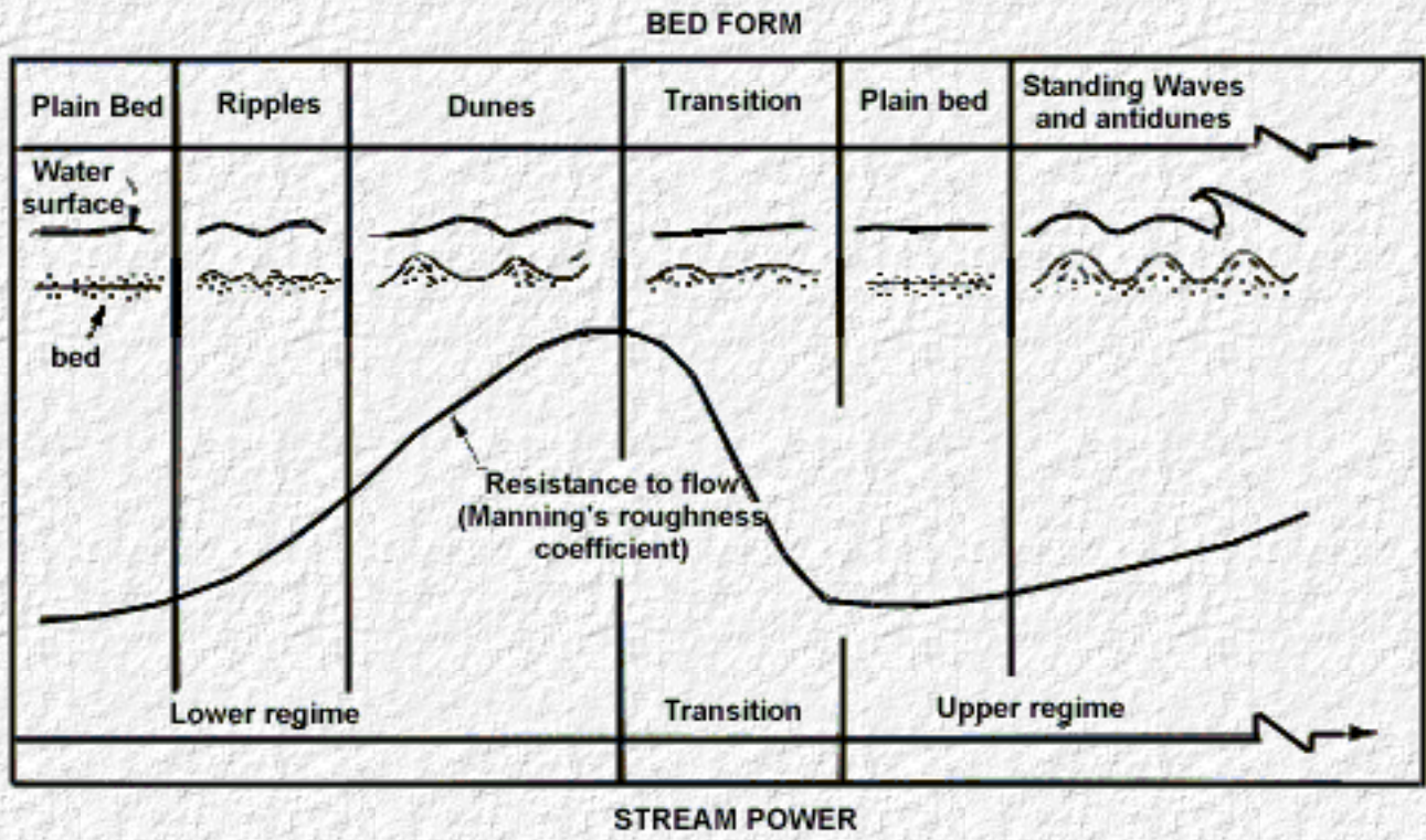
Figure 3. Forms and Bed Roughness in Sand-Bed Channels
