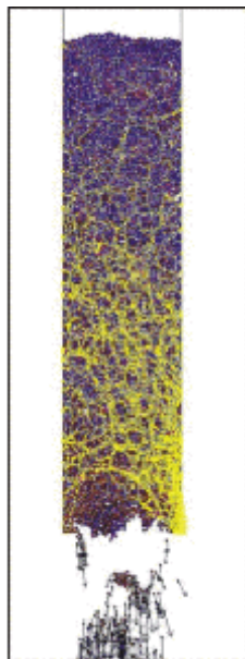
Cohesive forces and particle velocity vectors in a simulated ore pass.
