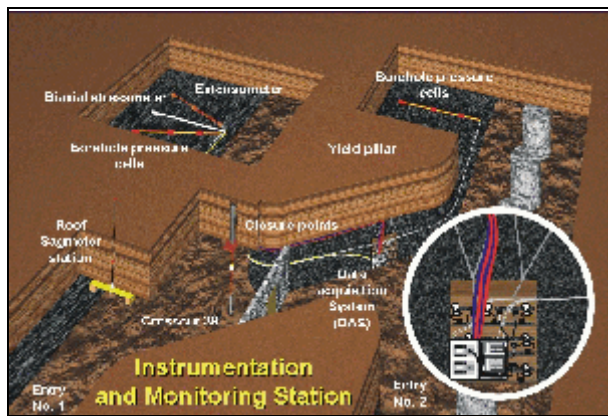
Stress monitoring system field tested for assessing coal bumps.
