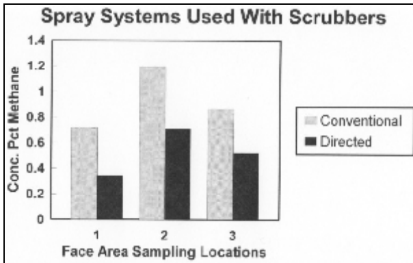
Modified spray system used with scrubber.
