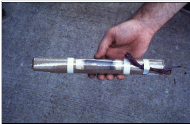
Explosive charge set up for the air gap test. This test evaluates the ability of the detonation of a permissible explosive to jump a gap in the explosive column.
