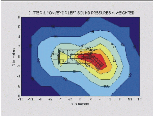
Noise profile for a continuous miner in free field, with the cutter and conveyor running.
