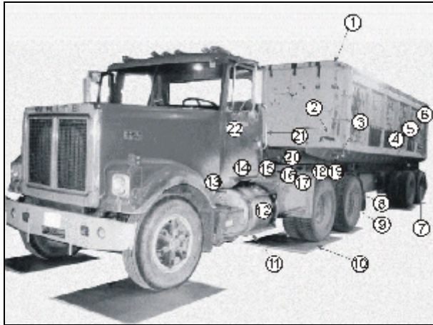
A 23-ton truck showing points used to measure voltage potentials that may be present on the exterior surface.
