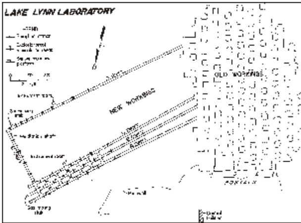
Experimental mine at Lake Lynn Laboratory.
