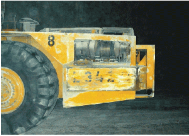
Diesel exhaust filtration on mining equipment offers substantial reductions in workplace DPM concentrations.
