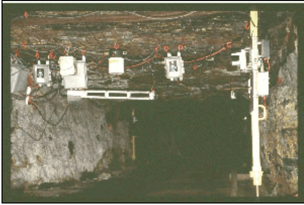
Mine fire sensor array in the Safety Research Coal Mine.
