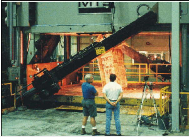
Safety performance testing of an innovative timber support in the Mine Roof Simulator.
