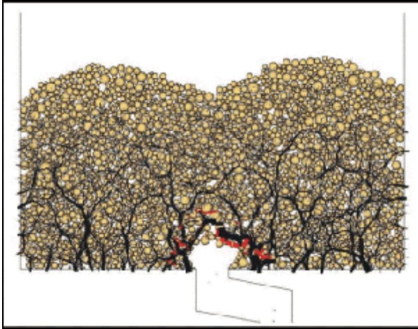
PFC model of a void forming above a feeder.
