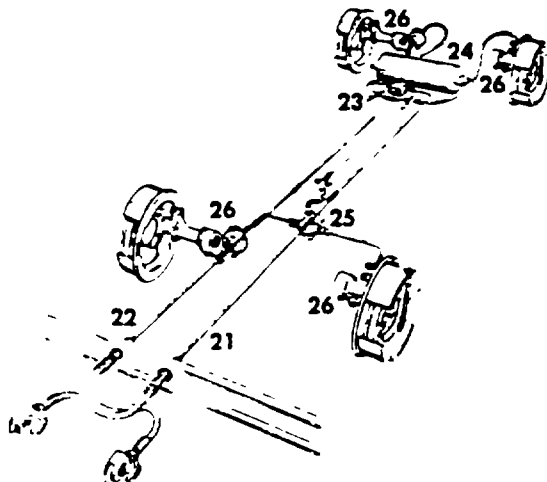
STRAIGHT AIR SYSTEM (Full Trailer)
