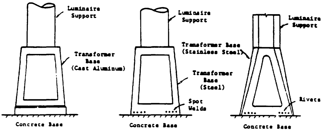
CAST ALUMINUM TRANSFORMER BASE (FRANGIBLE)
