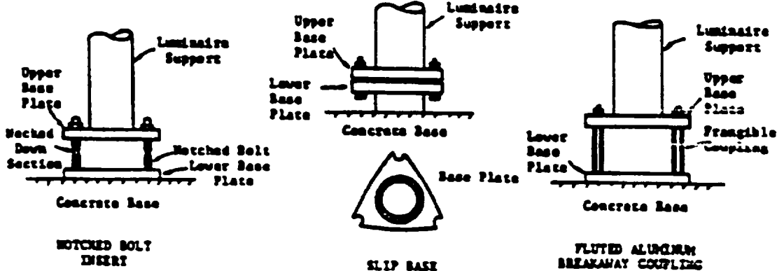
SLIP BASE
