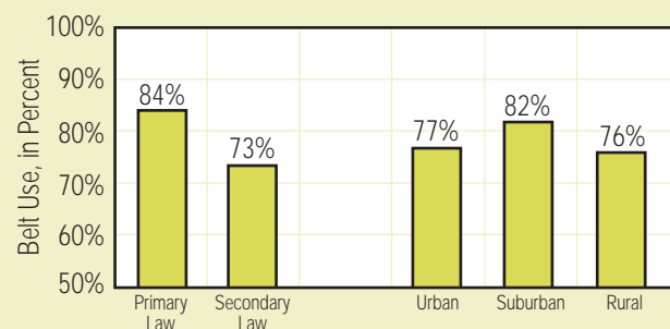
Safety Belt Use in 2004 by Law Type and Urbanization
