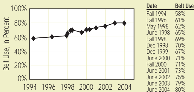
Safety Belt Use, 1994 — Present
