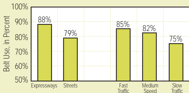
Safety Belt Use in 2004 by Road Type and Traffic Speed
