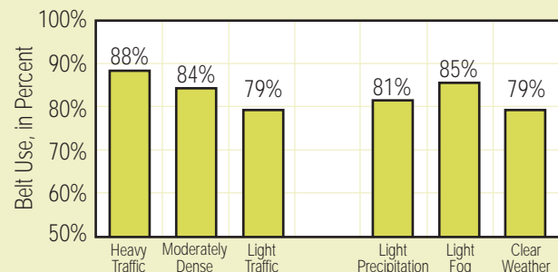
Safety Belt Use in 2004 by Traffic Density and Weather Conditions
