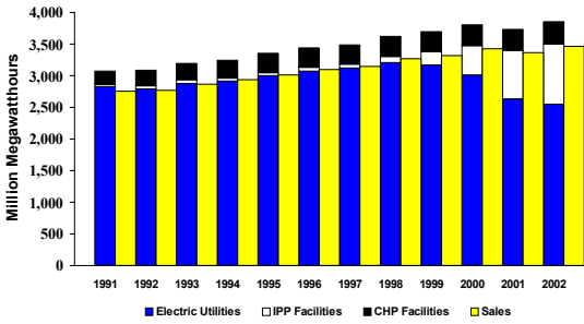
Figure 2: Total Net Generation Compared to Total Retail Sales, 1991- 2002
