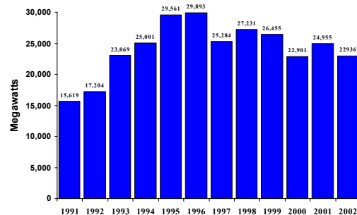
Figure 11: Demand-Side Management Peak Load Reductions, 1991-2002
