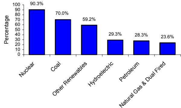
Figure 4: Average Capacity Factor by Energy Source, 2002
