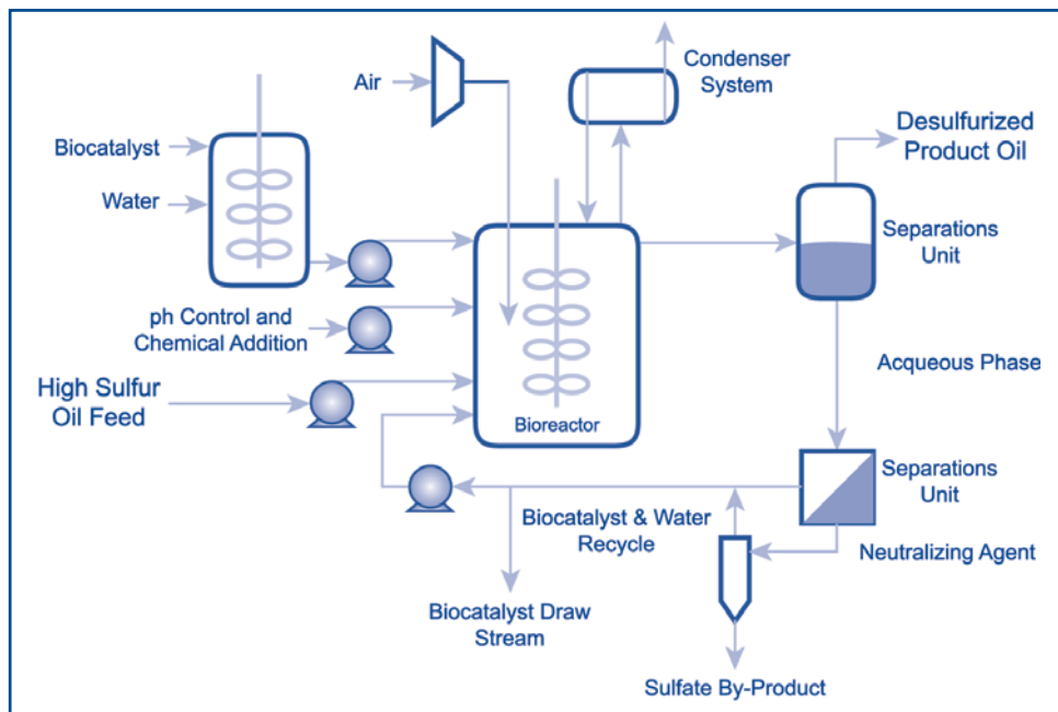
Preliminary bench-scale process design to test gasoline biodesulfurization.
