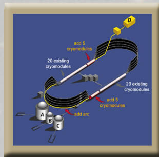
CEBAF 12 GeV Upgrade
