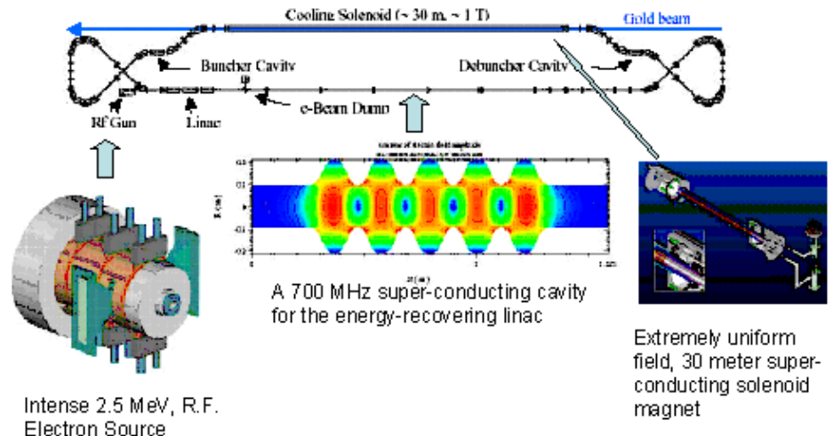
The RHIC II electron cooling system will enable RHIC to increase its collision rate 10-fold and maintain this collision rate for long periods of time.
