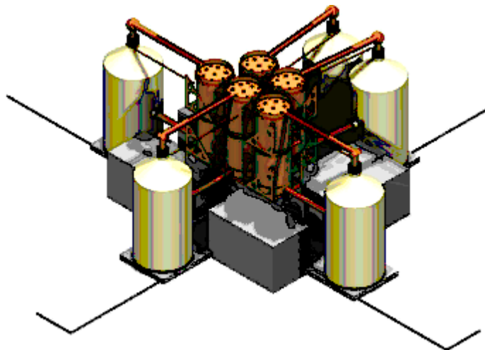
Artist's conception of one particular neutrino-less double beta decay experiment—the Majorana.
