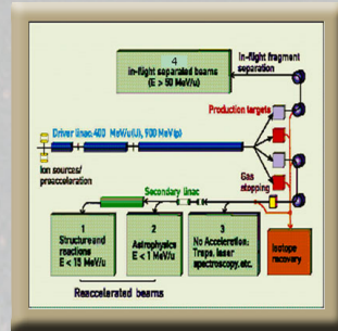
Rare Isotope Accelerator
