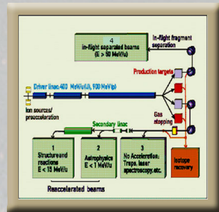
Rare Isotope Accelerator
