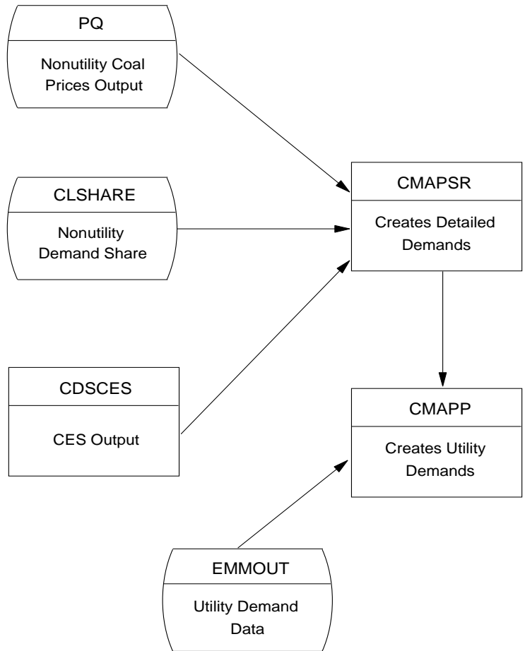
Figure 8. Functions of Subroutine “CMAPSR”
