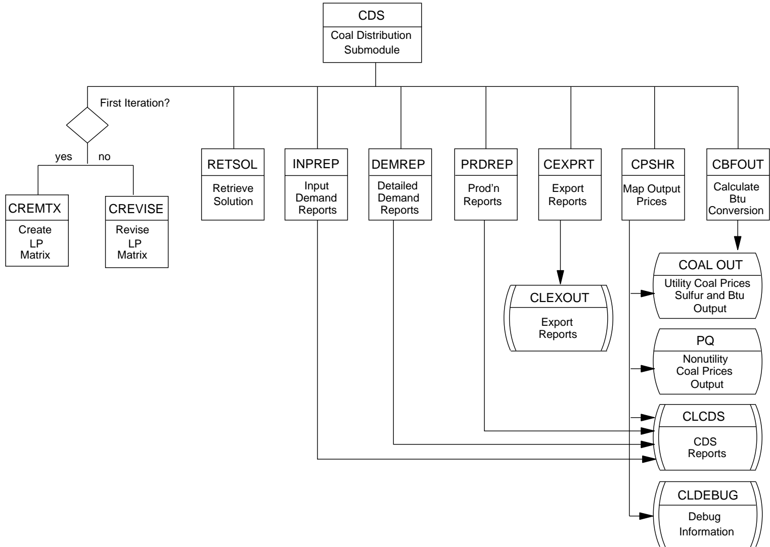
Figure 6. Calling Order for CDS Subroutines - Overview
