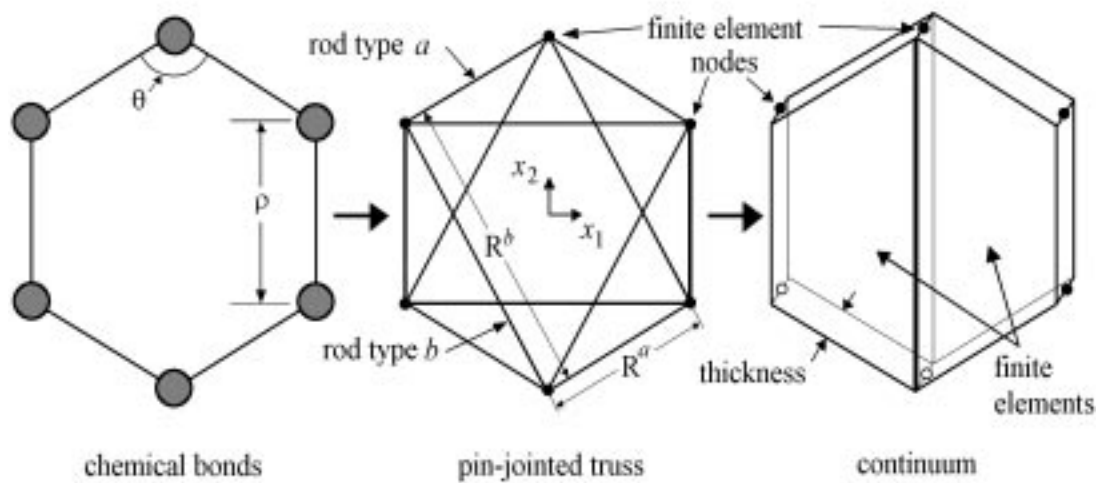
Figure 3 – Equivalent-continuum modeling of a graphene sheet.
