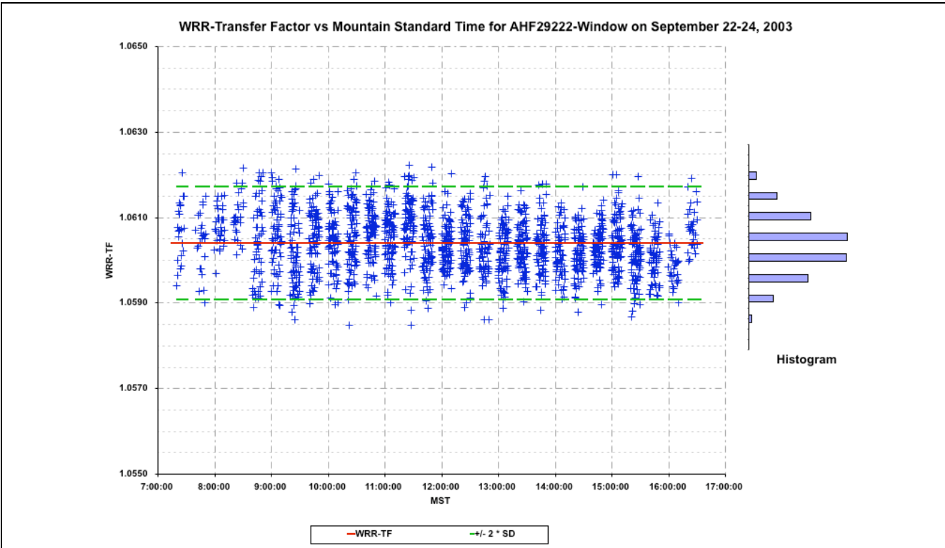
Figure 4.5.5 WRR Transfer Factor vs. Mountain Std Time for AHF29222-Window at NPC2003
