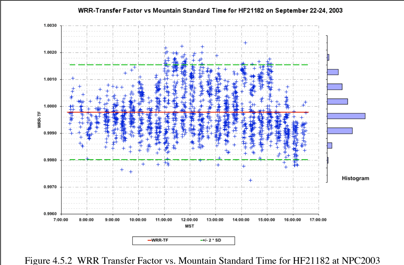
Figure 4.5.2 WRR Transfer Factor vs. Mountain Standard Time for HF21182 at NPC2003
