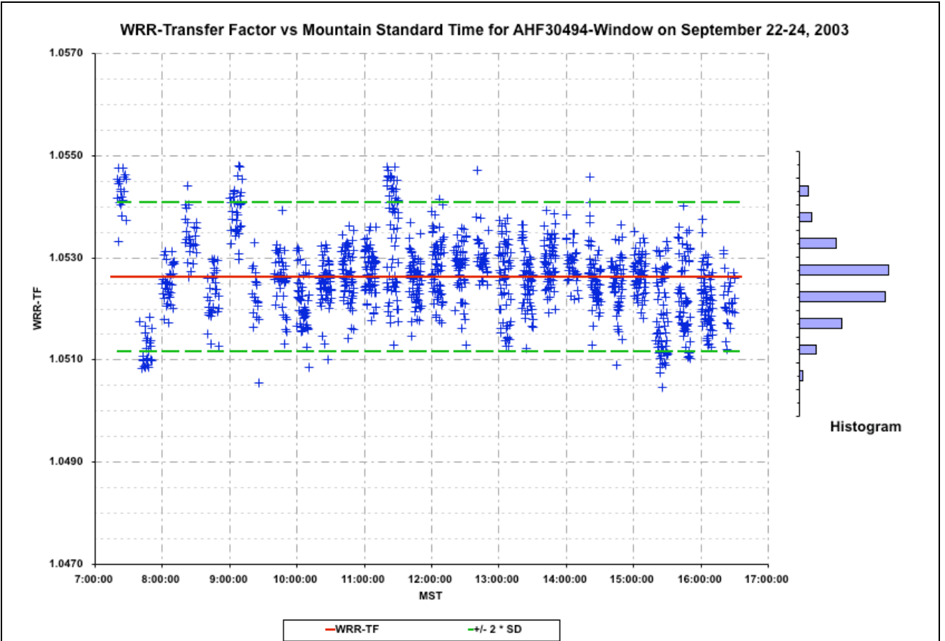
Figure 4.5.6 WRR Transfer Factor vs. Mountain Std Time for AHF30494-Window at NPC2003
