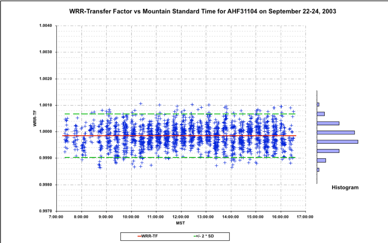
Figure 4.5.10 WRR Transfer Factor vs. Mountain Standard Time for AHF31104 at NPC2003
