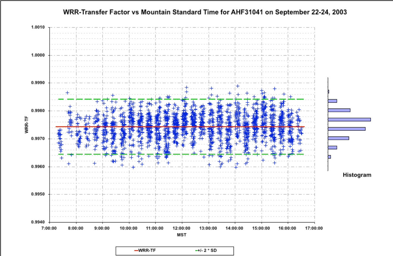
Figure 4.5.9 WRR Transfer Factor vs. Mountain Standard Time for AHF31041 at NPC2003
