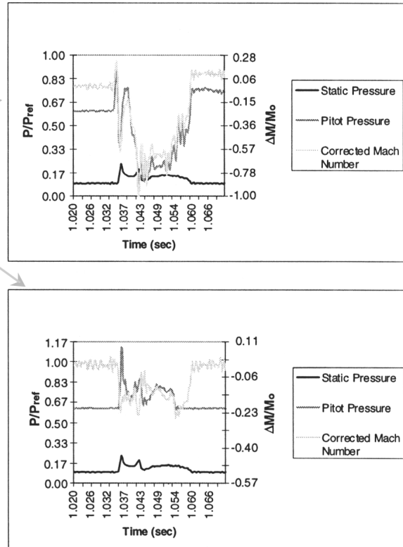
Figure 13. Local transient Mach number determined by flow field pressure measurements.
