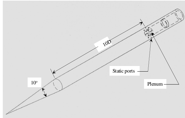
Figure 2. Sketch of static pressure probe tip.
