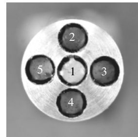
Figure 8. Front view of five-hole conical probe.
