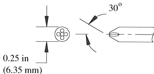
Figure 6. Schematic of five-hole conical probe.
