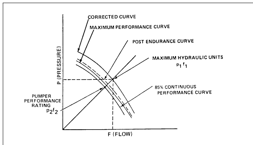
Figure 1. Pump performance curve.
