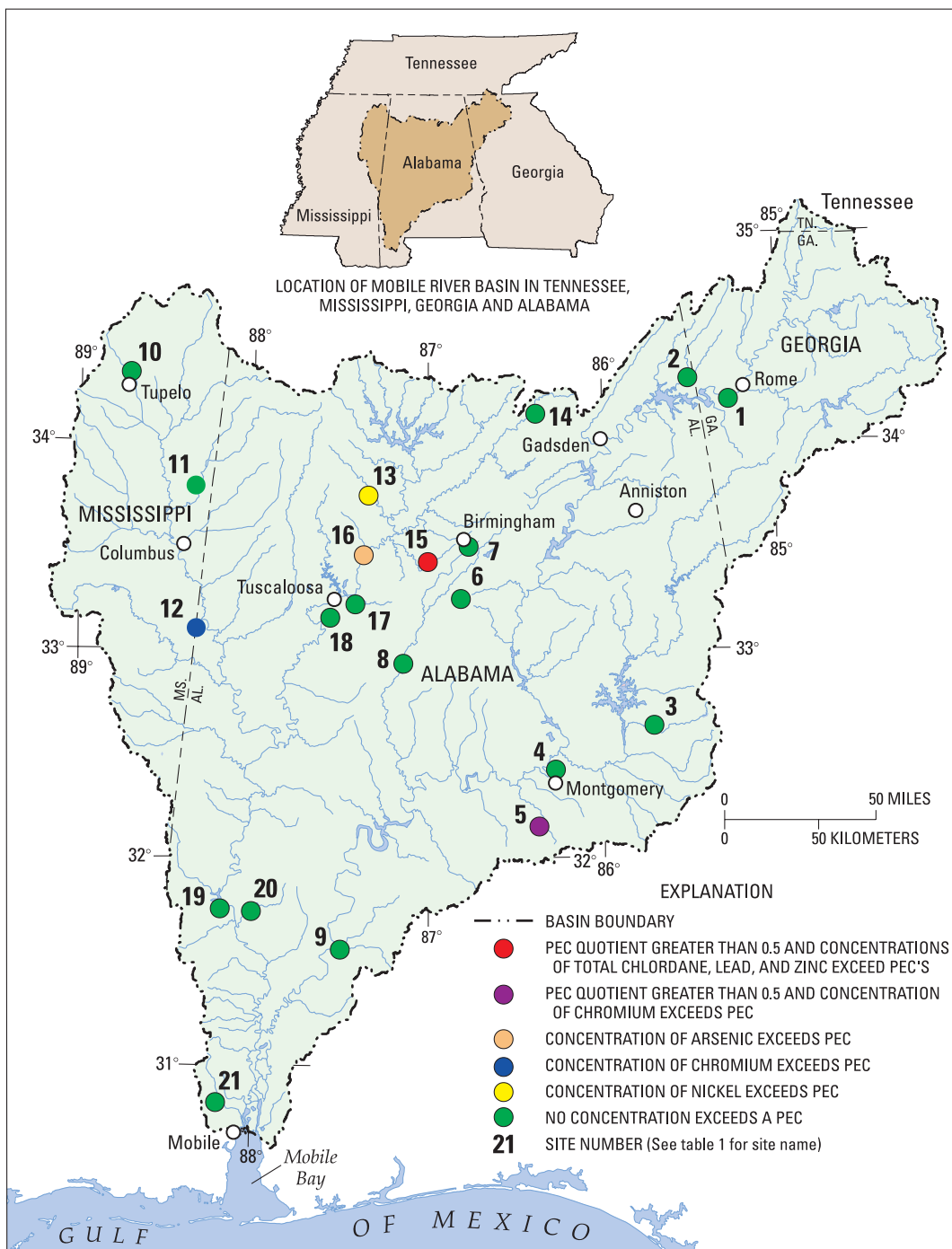
Figure 10. Sites in the Mobile River Basin where concentrations of organochlorine compounds and trace elements exceeded probable-effects concentrations and mean quotients in streambed-sediment samples.
