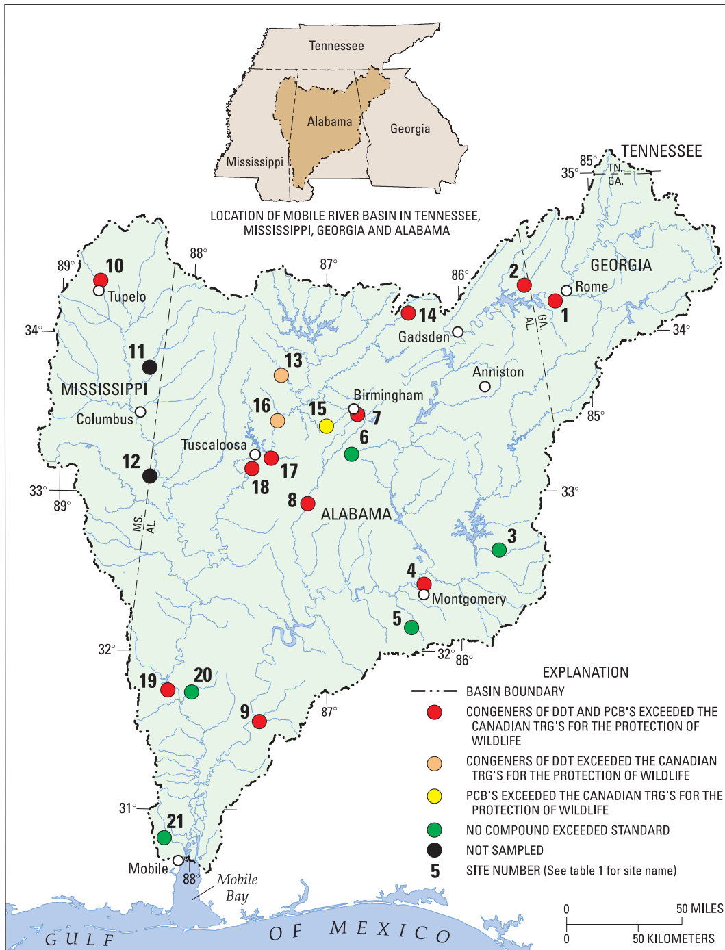
Figure 6. Sites in the Mobile River Basin where concentrations of organochlorine compounds in whole-fish tissue exceeded Canadian tissue residue guidelines (TRG's) for the protection of wildlife.
