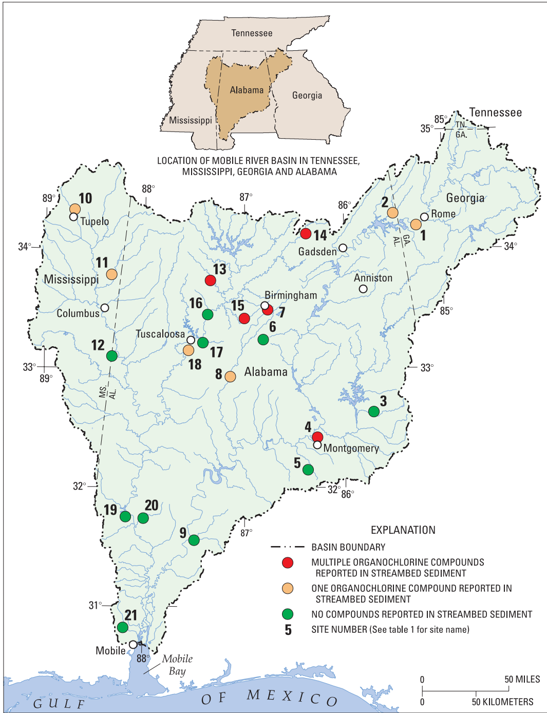
Figure 9. Sites in the Mobile River Basin where organochlorine compounds were reported in streambed- sediment samples.
