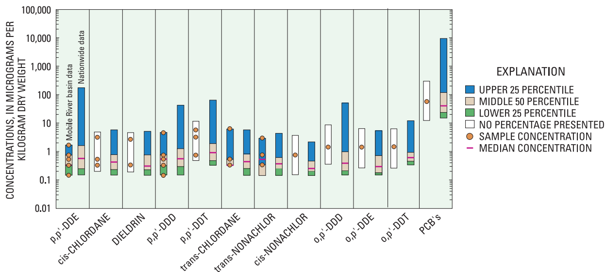
Figure 11. Floating bar charts of statistical distributions of concentrations of organochlorine compounds in streambed-sediment samples from the Mobile River Basin and in 1991 and 1994 National Water-Quality Assessment Program Study-Unit data.
