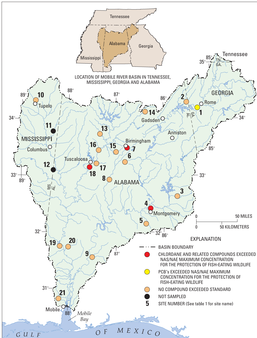
Figure 5. Sites in the Mobile River Basin where concentrations of organochlorine compounds in whole-fish tissue exceeded National Academy of Science and National Academy of Engineering guidelines for piscivorous wildlife.
