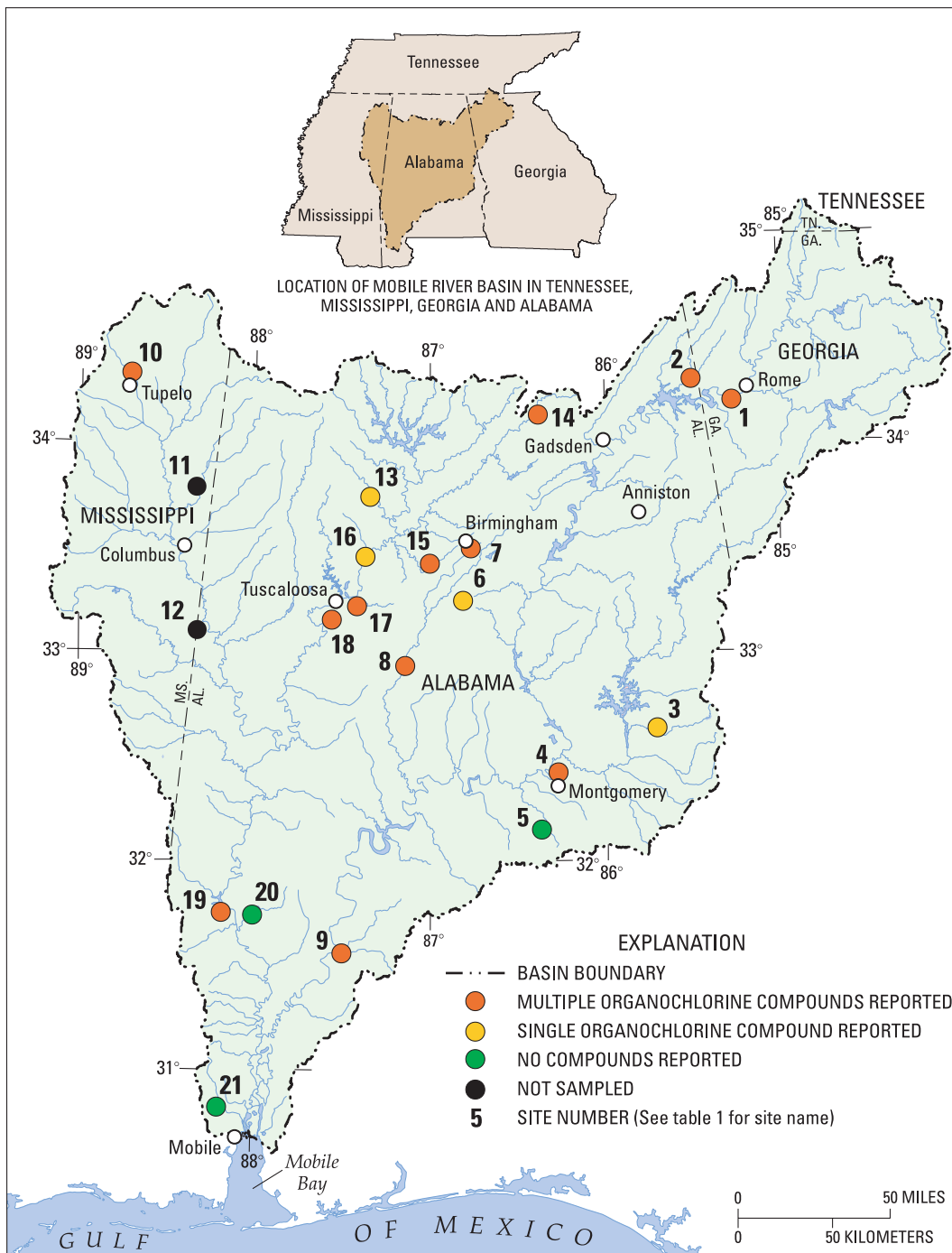
Figure 4. Sites where organochlorine compounds were reported in whole-fish tissue samples in the Mobile River Basin.
