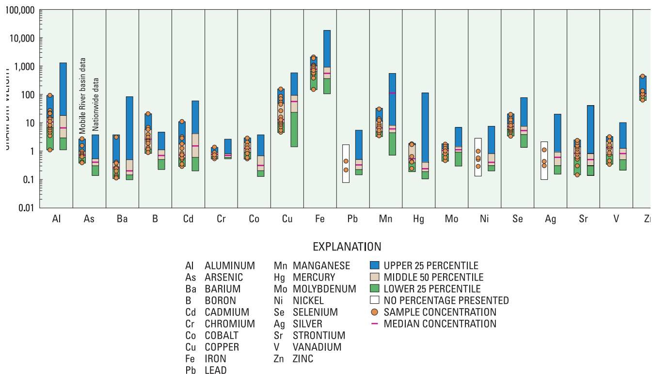
Figure 8. Floating bar charts of statistical distributions of concentrations of trace elements in fish-liver tissue samples from the Mobile River Basin and in 1991 and 1994 National Water-Quality Assessment Program Study-Unit data.
