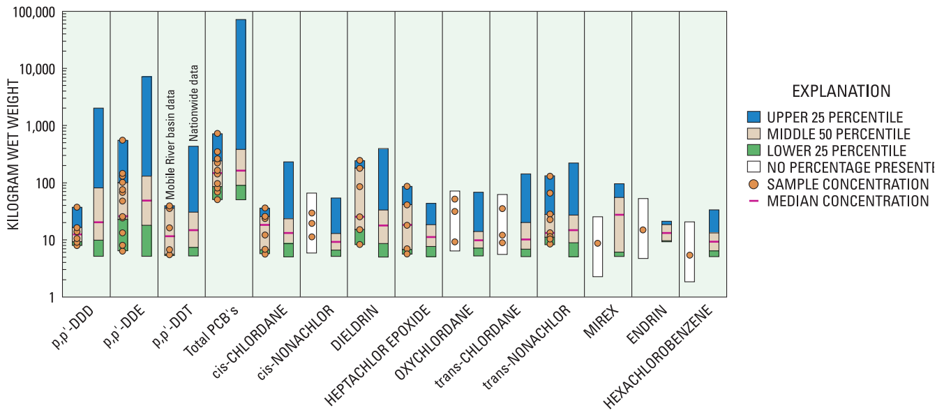
Figure 7. Floating bar charts of statistical distributions of concentrations of organochlorine compounds in whole-fish tissue samples from the Mobile River Basin and in 1991 and 1994 National Water-Quality Assessment Program Study-Unit data.
