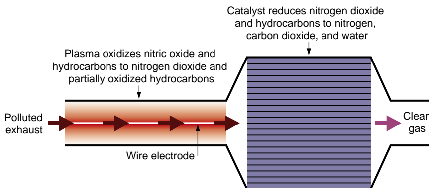
A schematic of the plasma-assisted catalytic reduction system. A nonthermal plasma is produced by short pulses of high voltage on a metal wire inside a metal cylinder.
