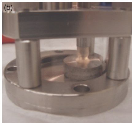
Livermore scientists have developed a new piercing device for extracting liquids under pressure in metal capsules following gas-gun shock experiments. (a) The piercing device consists of a clean glass chamber between two metal plates. The top plate has a connection for a drill bit and a silicon septum through which a needle can pass for sample collection. (b) A shocked capsule is positioned in the piercer under the drill. A Teflon sleeve around the drill bit will capture any spray that occurs when the capsule is punctured. (c) The capsule has been pierced and the drill retracted. Shocked liquid has beaded on the surface of the capsule awaiting collection.
