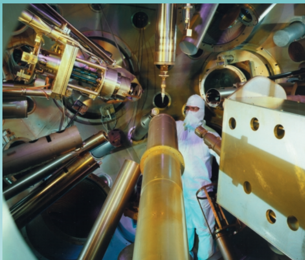
Inside the main chamber of Nova (the predecessor system to the National Ignition Facility), diagnostics surround the target mounted at the end of the rod in the chamber’s center.
