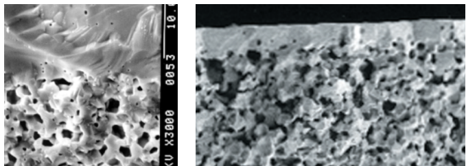
This cross section of yttria-stabilized zirconia electrolyte, imaged at different resolutions, is an example of a thin film that was deposited on a porous anode using colloidal spray deposition.
