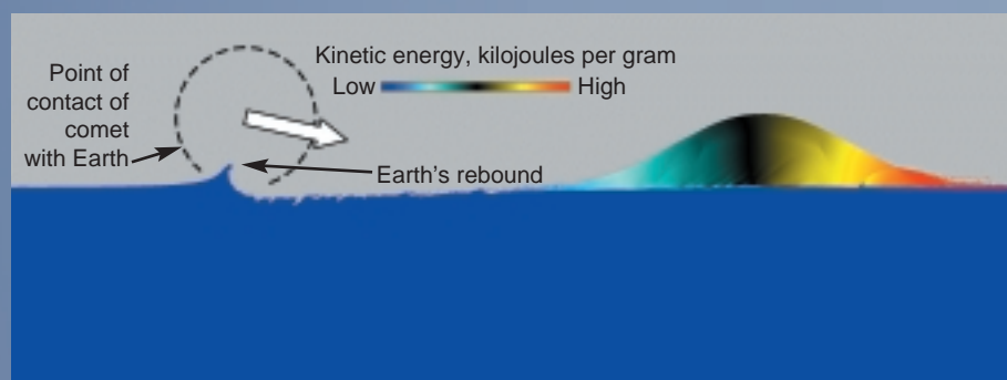
A two-dimensional simulation of an icy comet hitting the rocky Earth. This image represents the distribution of kinetic energy 678 microseconds after impact, sufficient time for the primary shock wave to pass completely through the comet. The wide distribution of energy in the comet indicates that the comet's trailing portion should be cooler—and experience lower velocity—than the front end. Thus, the rear part of the comet could arrive as a puddle of liquid water, with a high concentration of organic compounds, ready to host further chemical evolution. (Simulation by Greg Miller, Lawrence Berkeley National Laboratory.)
