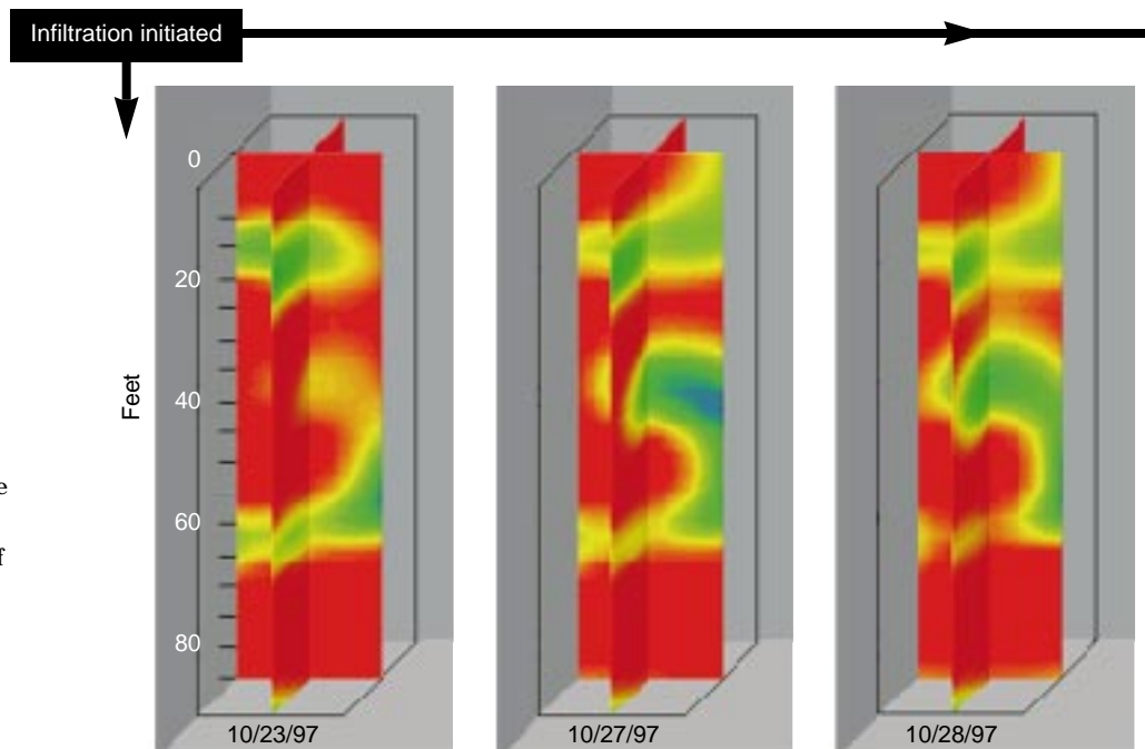
Figure 3. Several days following the start of the infiltration experiment, resistivity changes are apparent at the 40-foot level in the vadose zone. Oscillations in colors also occur (red = no resistivity change, blue = most negative resistivity change, or greater saturation). These changes in saturation result from the periodic upward flow of air in the vadose zone along permeable channels in a manner similar to the periodic flow of air through a narrow-necked, water-filled bottle turned upside down.
