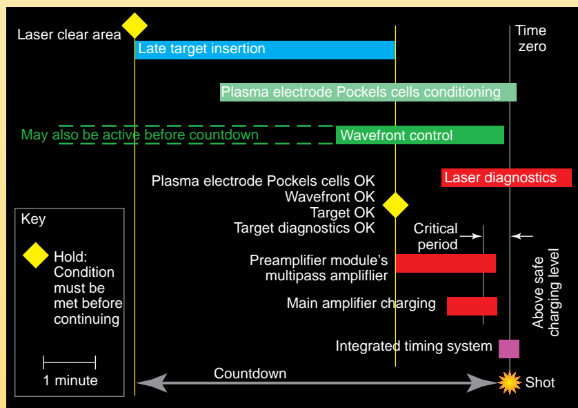
During the final 5- to 7-minute countdown before a NIF laser shot, all operations that must occur before the shot can happen are reviewed by the control system and precisely sequenced.
