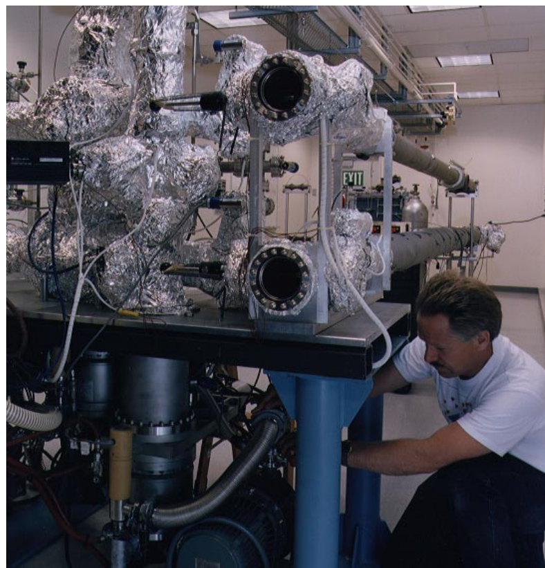
Figure 6. Livermore engineers clean nearly a kilometer of 2.4-meter (8-foot-) long straight sections of beam pipes through a process called glow-discharge cleaning that rids the metal of residual carbon and contaminants. Here, Fred Holdener works with a vacuum pump prior to cleaning operations.
