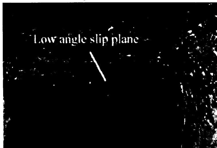
Photograph of a low-angle slip plane that created an unstable roof wedge.
