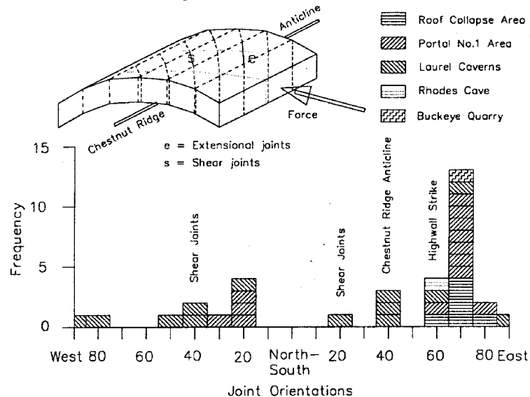
A histogram of major joint orientations in the Loyalhanna formation near the Lake Lynn Laboratory, showing the relationship between orientation and structural folding of stone bearing strata.
