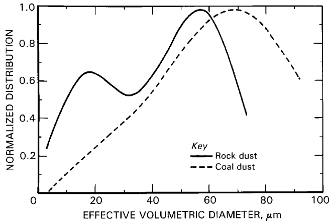
Figure 1.—Normalized particle size distribution of both coal and rock dust.
