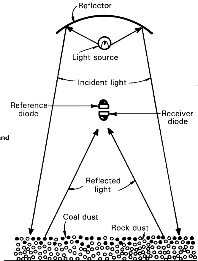
Figure 2.—Principle of operation of float dust deposition meter.
