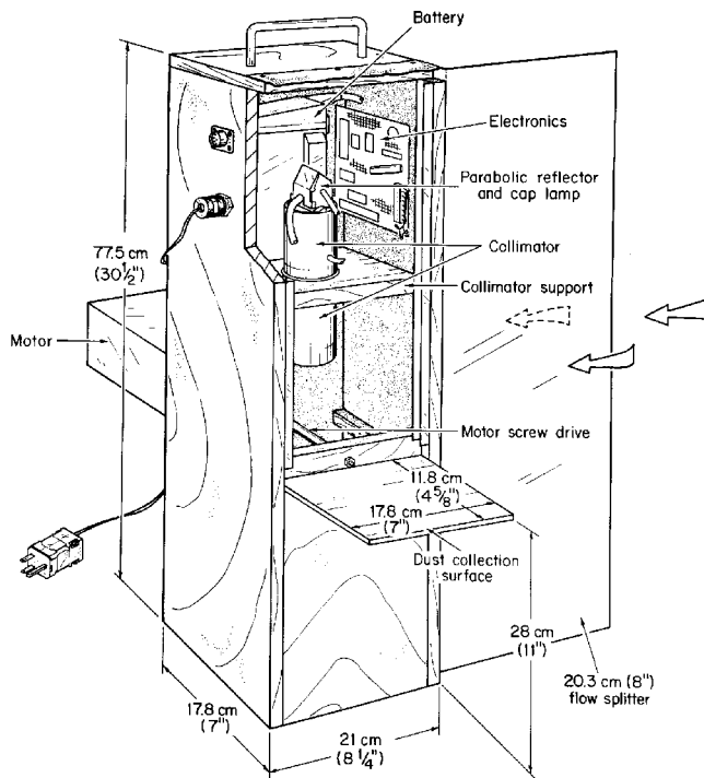
Figure 4.—Float dust deposition meter used during full-scale studies at the Lake Lynn Experimental Mine.
