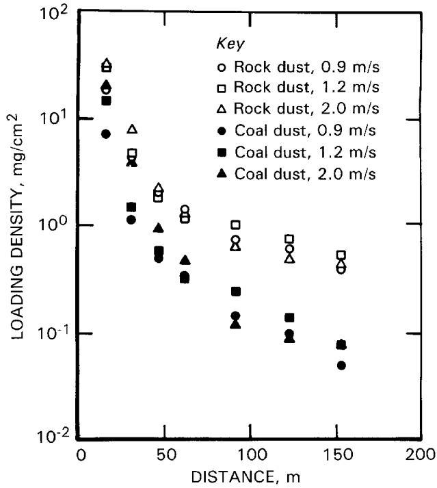
Figure 7.—Loadings of coal and rock dust deposited at various distances downwind of the dust source for three ventilation velocities.
