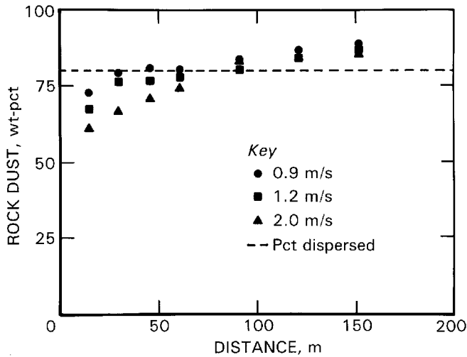
Figure 8.—Wt-pct of rock dust deposited as a function of distance from the dust source for three ventilation velocities.
