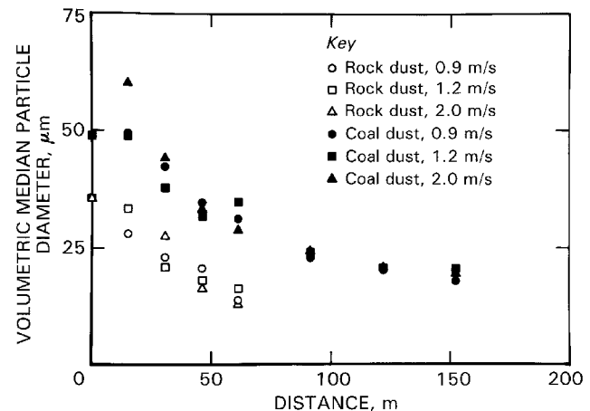
Figure 6.—Unagglomerated volumetric median particle diameters of coal and rock dust deposits as a function of distance downwind of the dust source.
