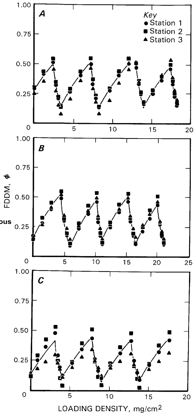
Figure 9.—Float dust deposition meter ( \Phi ) versus loading density, as measured from the petri dishes, with fitted theory \Phi for 0.9 m/s ( \alpha_c = 1.38 and \alpha_r = 0.15 cr/mg), 1.2 m/s ( \alpha_c = 1.27 and \alpha_r = 0.13 cr/mg), and 2.0 m/s ( \alpha_c = 1.40 and \alpha_r = 0.13 cr/mg).
