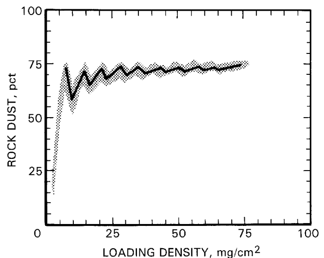
Figure 10.—95% confidence band of total mass fraction as a function of the combined rock dust/coal dust loading density over a simulated 10 cycles.
