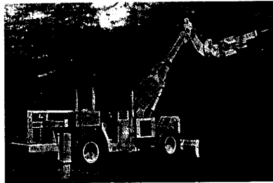
Figure 7. Hammer-type scaler.
