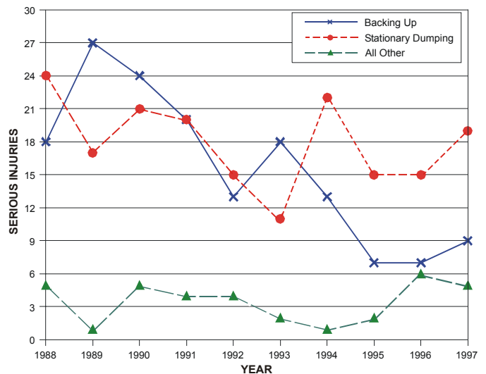
Figure 7.—Serious injuries by haulage truck activity, 1988-1997.
