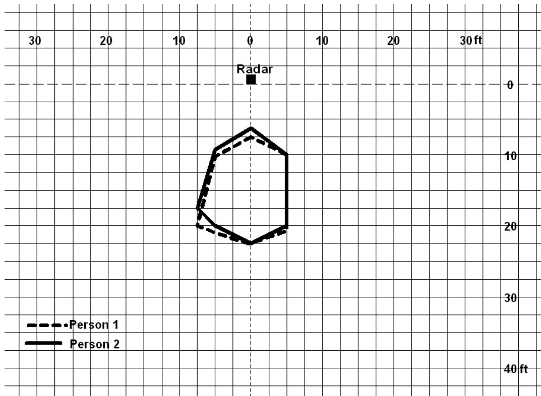
Figure 20.—Detection zones for persons 1 and 2 and system 1 mounted high (25° tilt).
