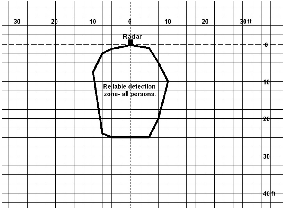
Figure 17.—Detection zones for persons 1, 2, and 3 and system 1 mounted low.
