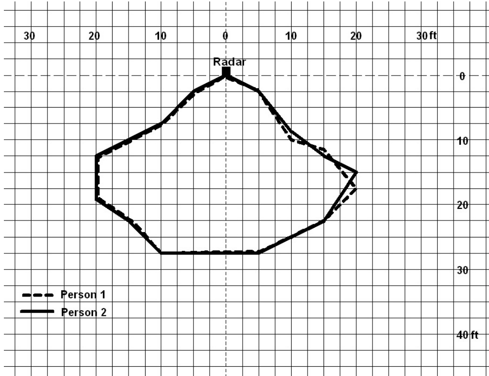
Figure 21.—Detection zones for persons 1 and 2 and system 2 mounted low.
