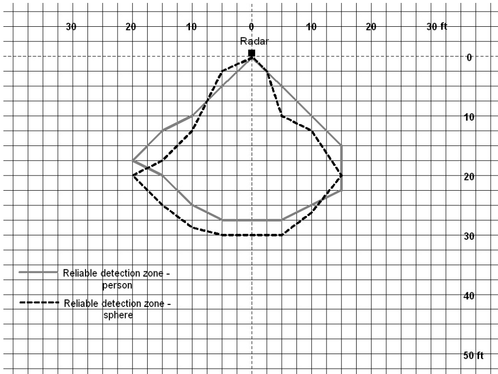
Figure 12.—System 2: Detection zones for person and large sphere.
