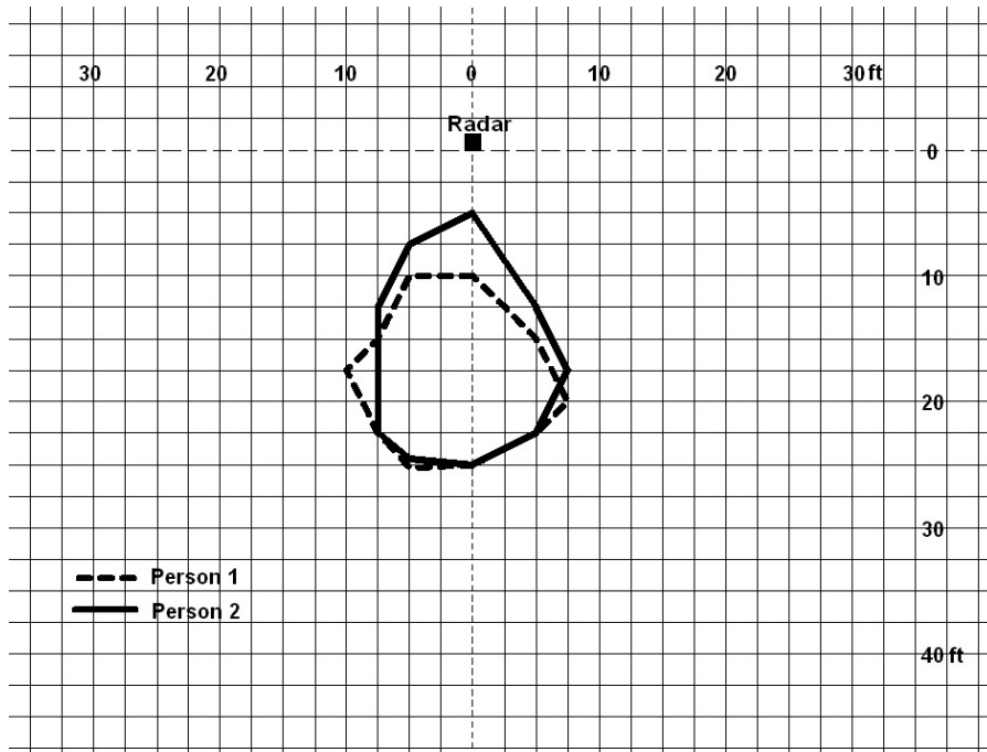
Figure 18.—Detection zones for persons 1 and 2 and system 1 mounted high (15° tilt).
