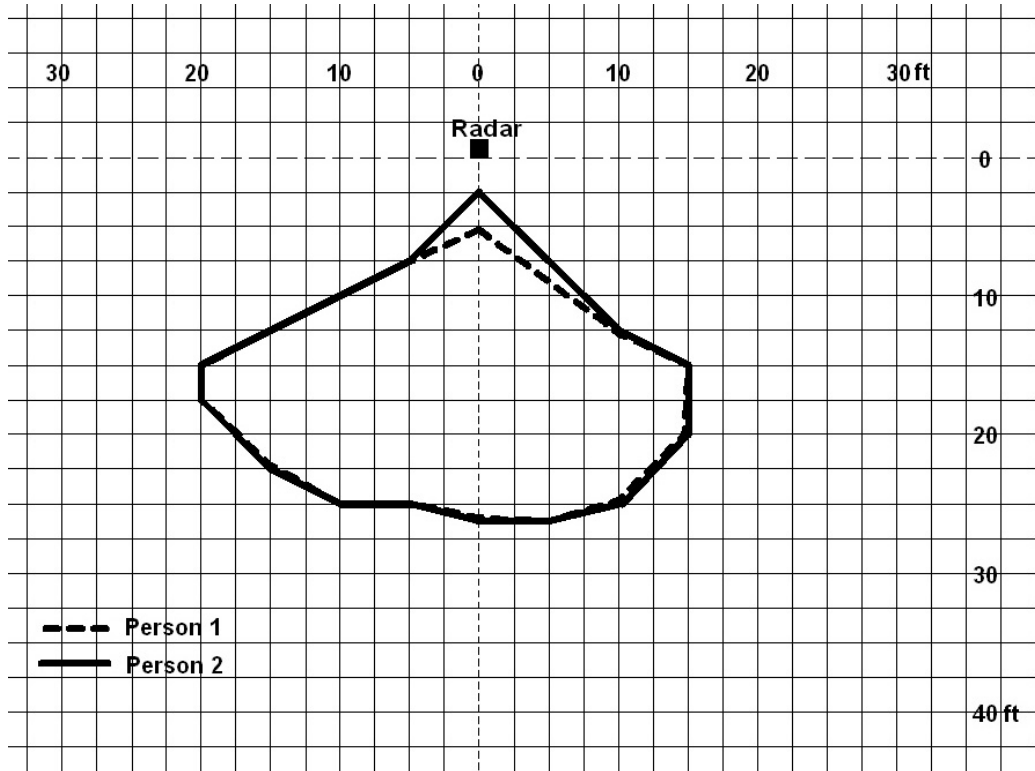
Figure 23.—Detection zones for persons 1 and 2 and system 2 mounted high (25° tilt).
