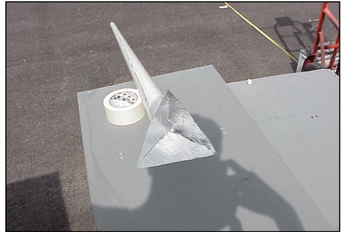
Figure 1.—Small trihedral corner reflector attached to PVC pipe.
