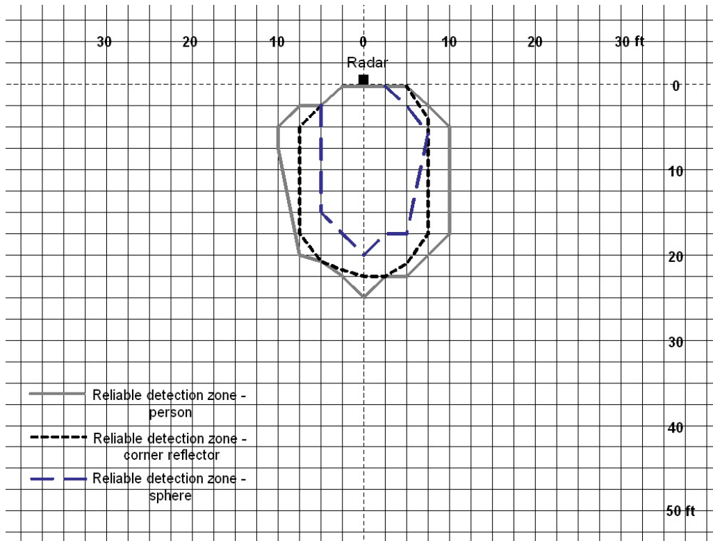
Figure 9.—System 1: Detection zones for person, corner reflector, and small sphere.
