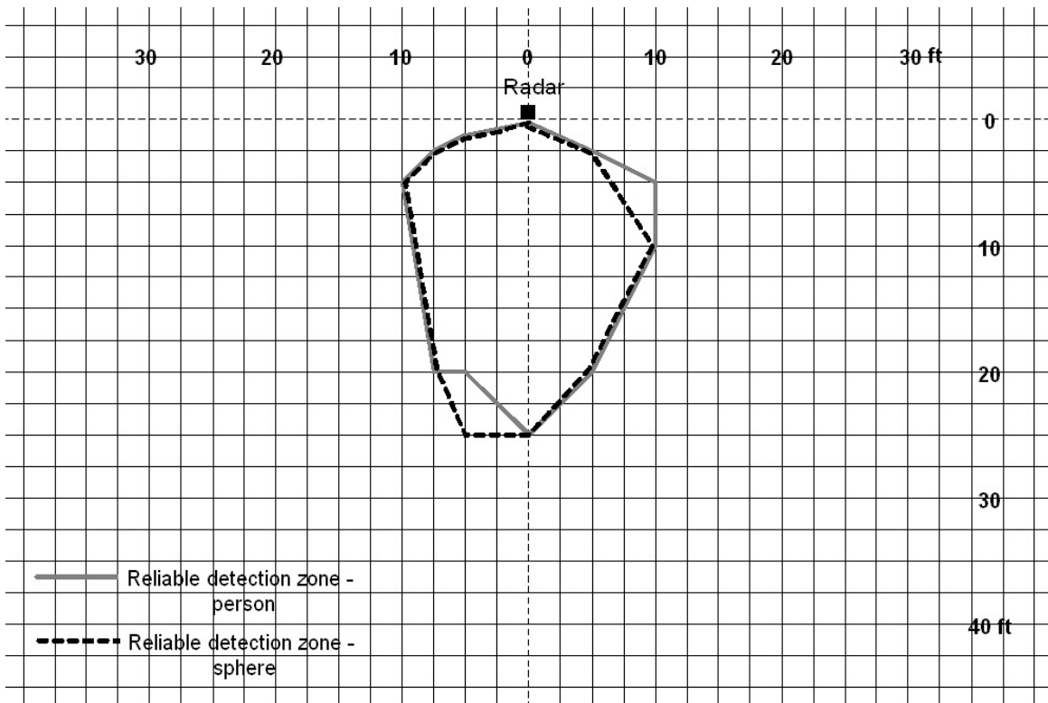
Figure 10.—System 1: Detection zones for person and large sphere.
