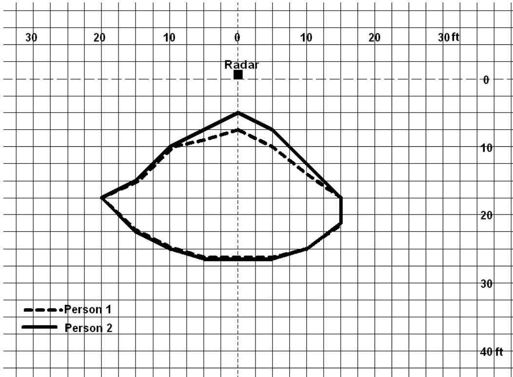
Figure 22.—Detection zones for persons 1 and 2 and system 2 mounted high (15° tilt).
