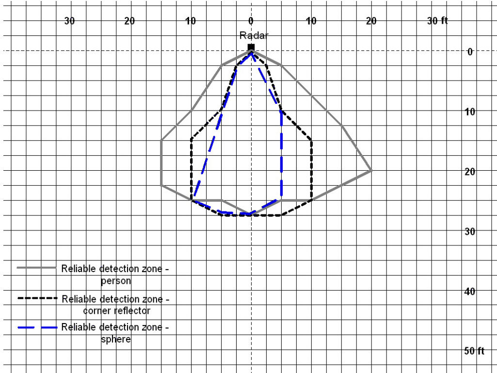
Figure 11.—System 2: Detection zones for person, corner reflector, and small sphere.
