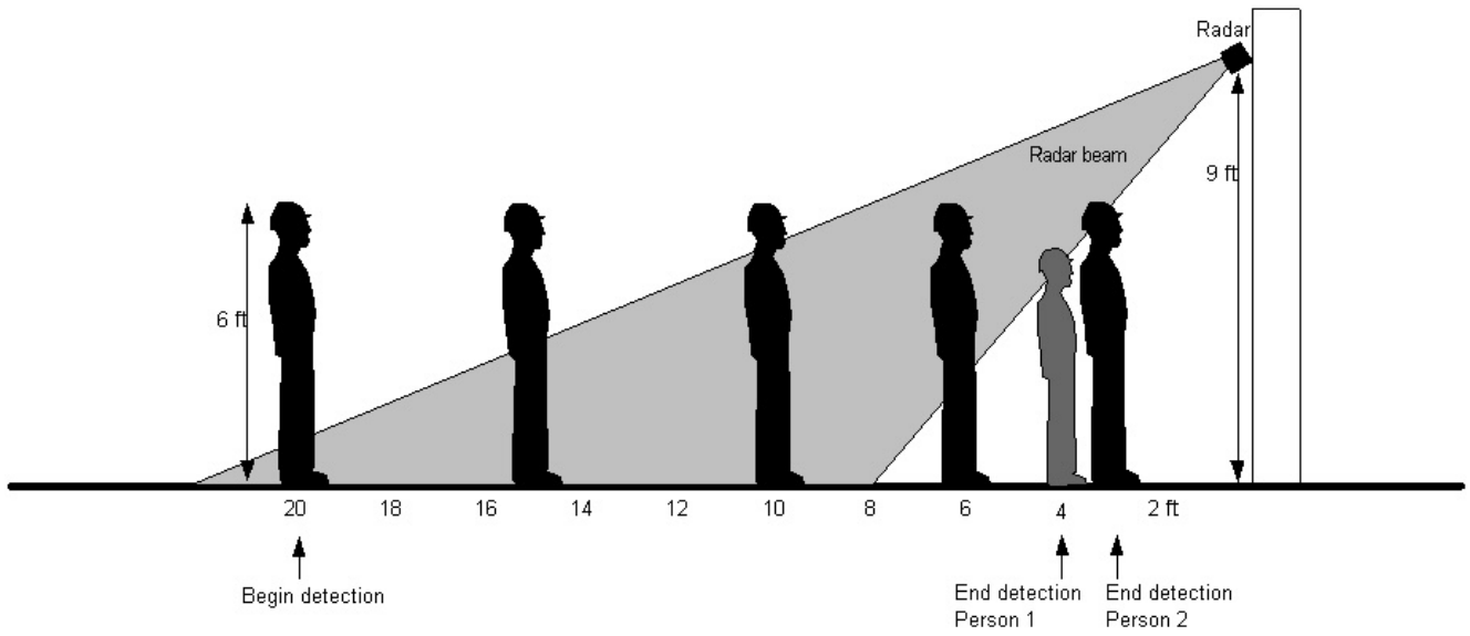
Figure 19.—Example of differences in inner detection ranges.
