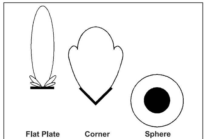
Figure 2 —Approximate radar cross-section patterns for different reflectors with relative magnitudes of reflected signal (U.S. Dept. of the Navy, 2001).
