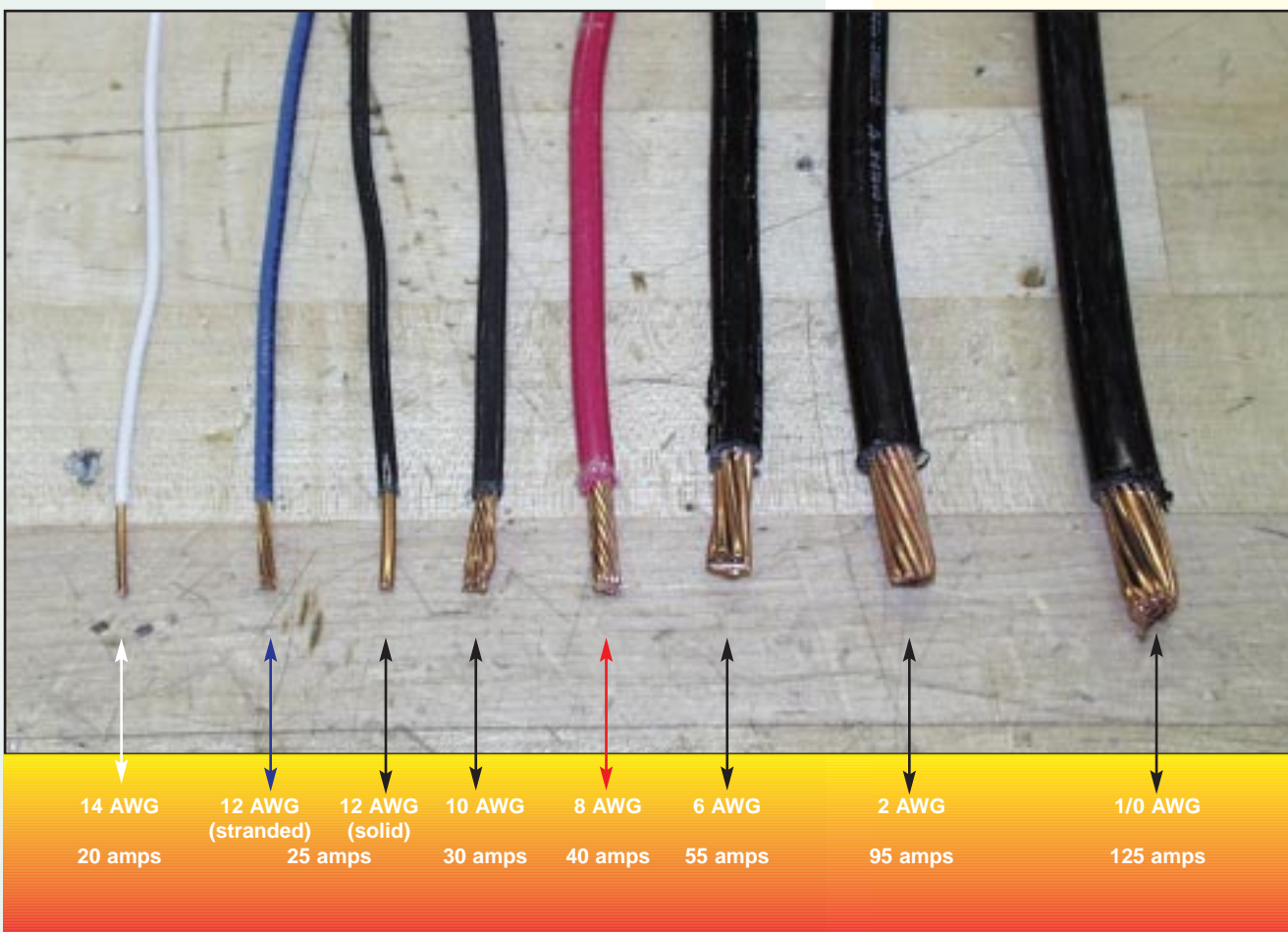
Wires come in different sizes. The maximum current each size can conduct safely is shown.
