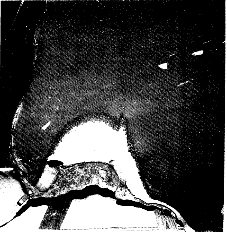
Right Hand SRM Segment Showing Erosion From Hot Propellant Gas (Lower Section)
