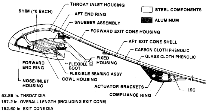
Figure 9. SRM Bolt-On Nozzle
