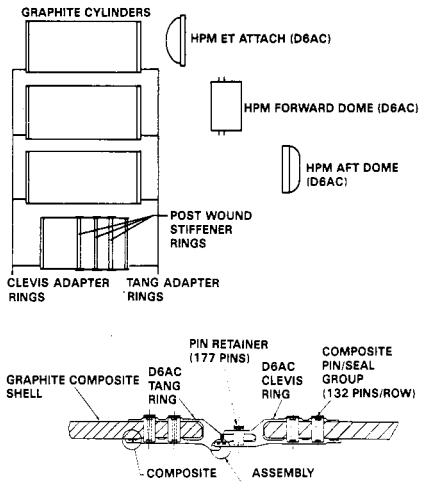
Figure 11. FWC-SRM Case Segments
