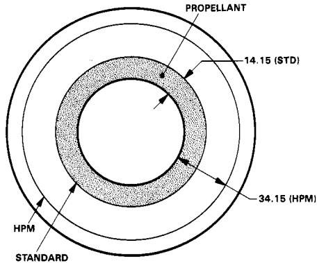
Figure 7. Center Segment Propellant Inhibitor Patterns
