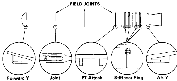
Figure 10. SRM Case
