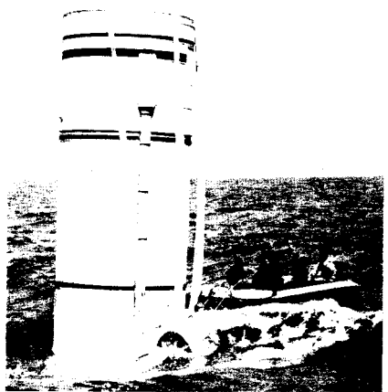
Figure 25. SRB in Spar Mode
