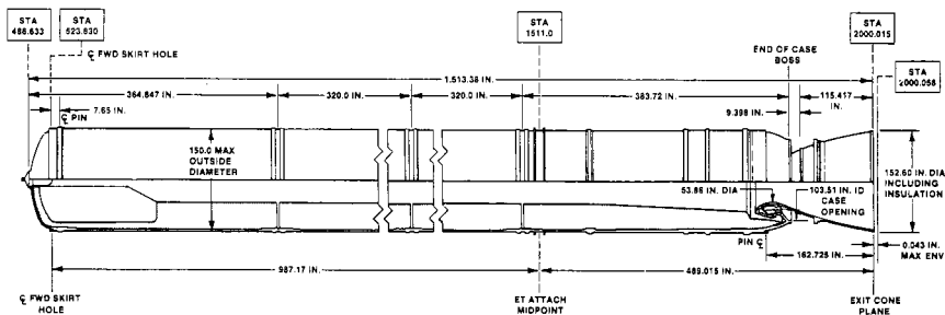
Figure 14. FWC-SRM Design Configuration
