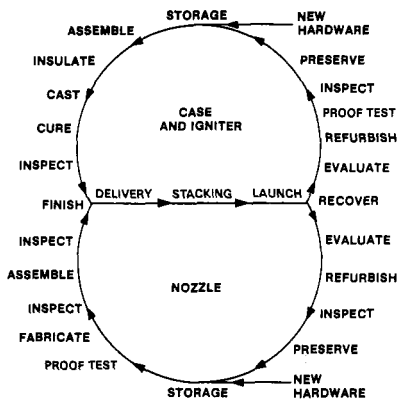
Figure 27. SRM Hardware Mission Cycle
