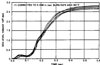
Figure 16. Composite of 26 SRM Thrust-Time Traces During Ignition
