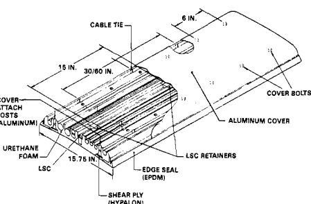
Figure 13. Systems Tunnels
