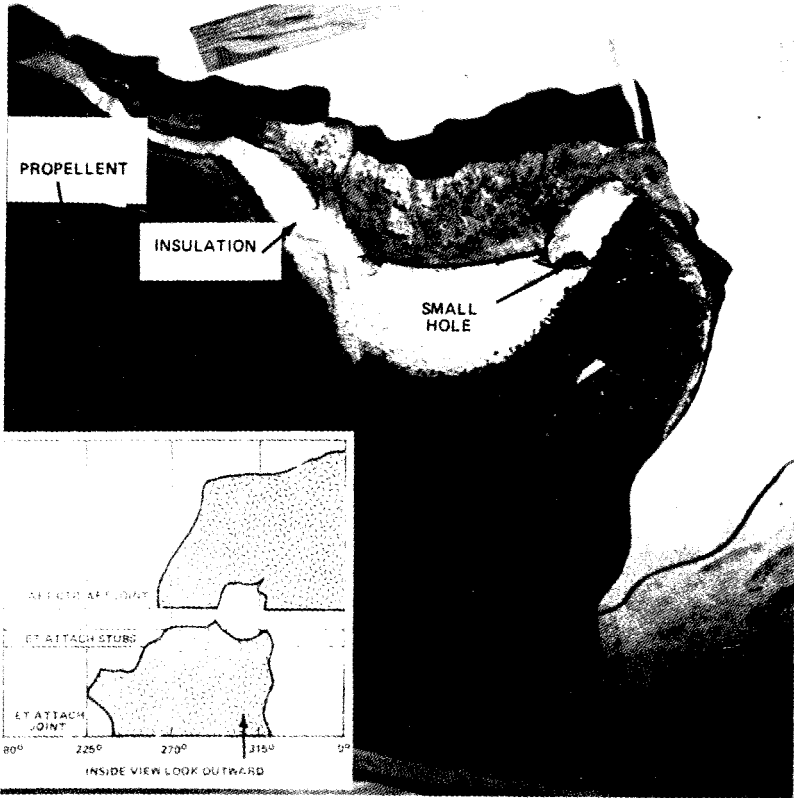
Recovered Portion of SRM Aft Segment
