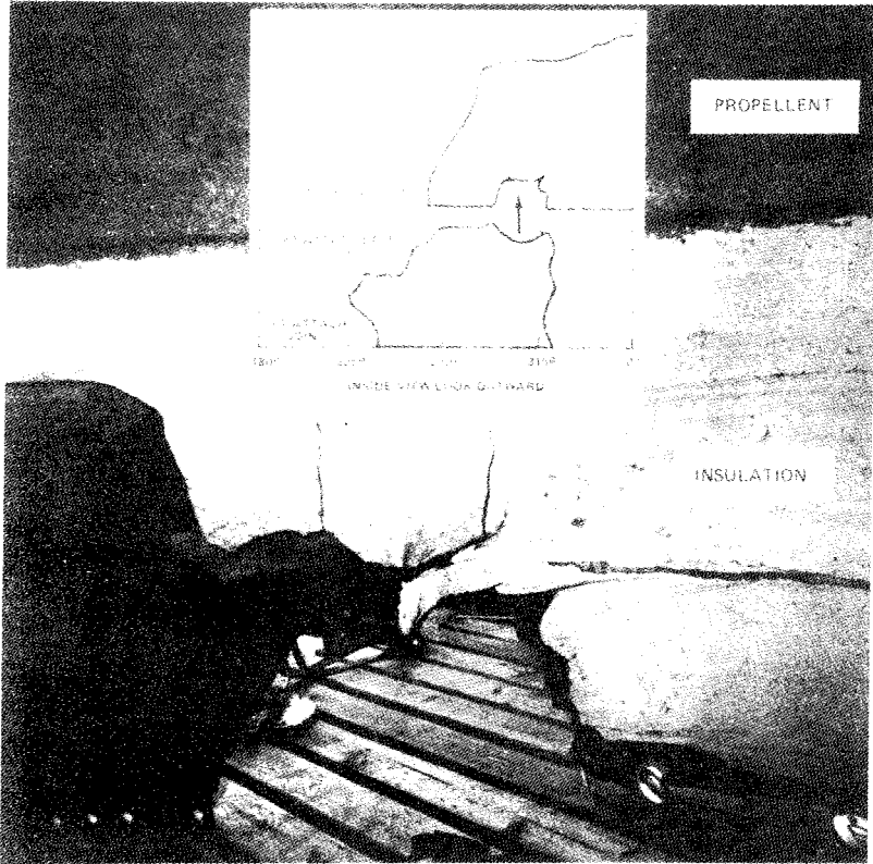
Reversed Portion of SRM Aft Center Segment
