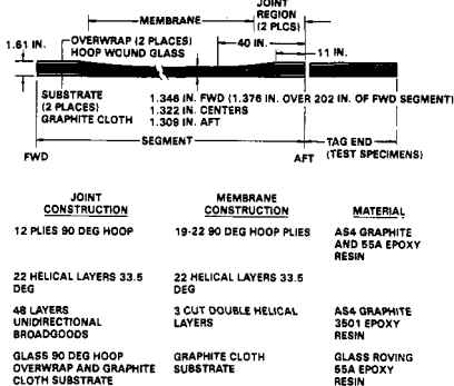
Figure 12. Typical Composite Segment Construction
