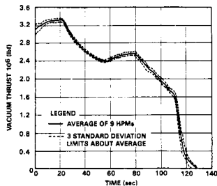
Figure 17. Thrust-Time Trace Reproducibility Experience
