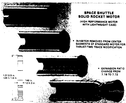
Figure 3. SRM Casting Segments
