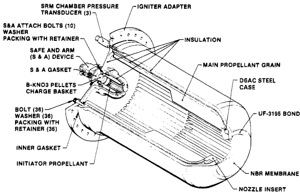
Figure 8. SRM Igniter
