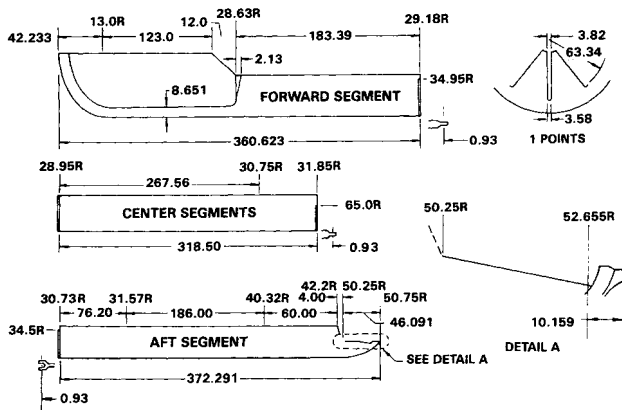
Figure 4. HPM Grain Configuration
