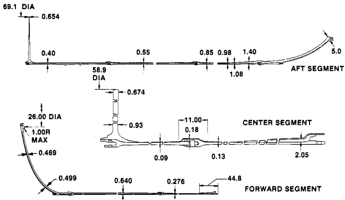
Figure 6. HPM Insulation Design
