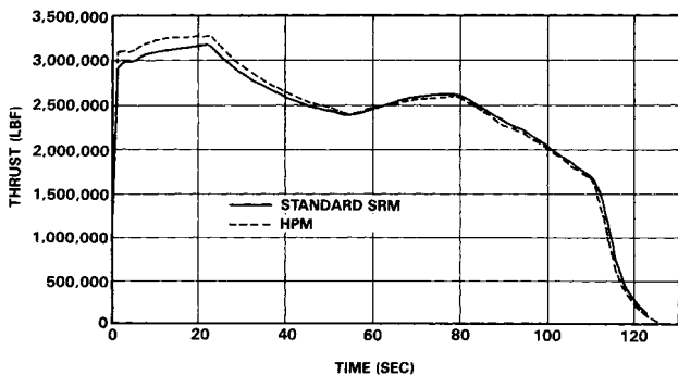
Figure 5. Thrust-Time Comparison, Standard SRM vs HPM
