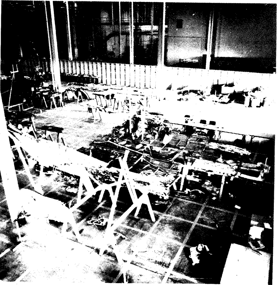
Orbiter Wreckage Layout
