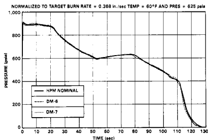
Figure 15. Pressure vs Time
