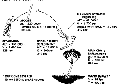
Figure 19. Typical SRB Reentry Profile
