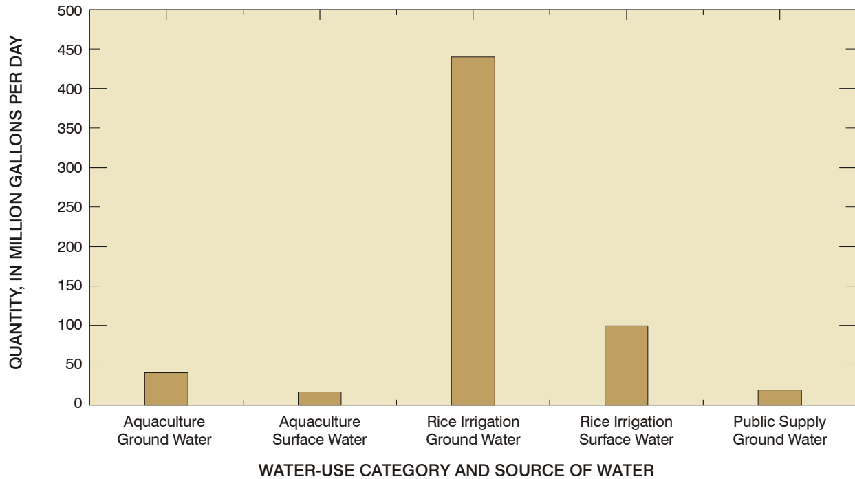
Figure 5. Sources and quantities of water used in the Mermentau River Basin, southwestern Louisiana, 2000.
