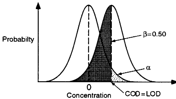
Figure 4-2. Graphic depiction of the relationship between the criterion of detection (COD), \alpha and \beta when COD = LOD .
