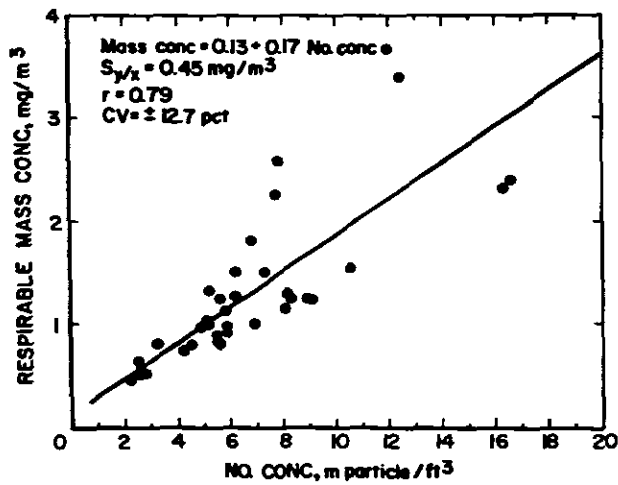
Figure 3. Comparison of dust concentrations obtained from midget impinger and respirable mass dust samples at two talc processing operations.
