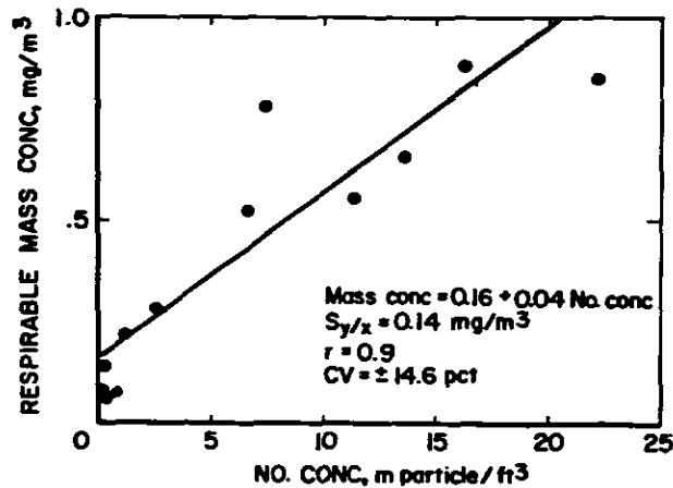
Figure 4. Comparison of dust concentrations obtained from midget impinger and respirable mass dust samples at two diatomaceous earth processing operations.
