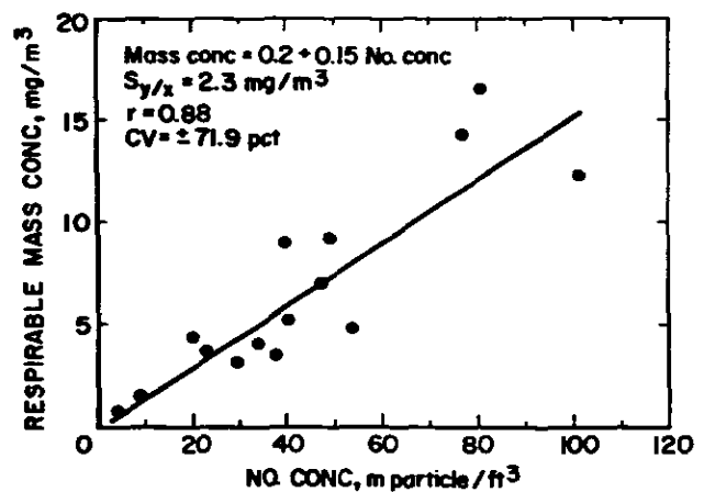
Figure 5. Comparison of dust concentrations obtained from midget impinger and respirable mass dust samples at two mica processing operations.
