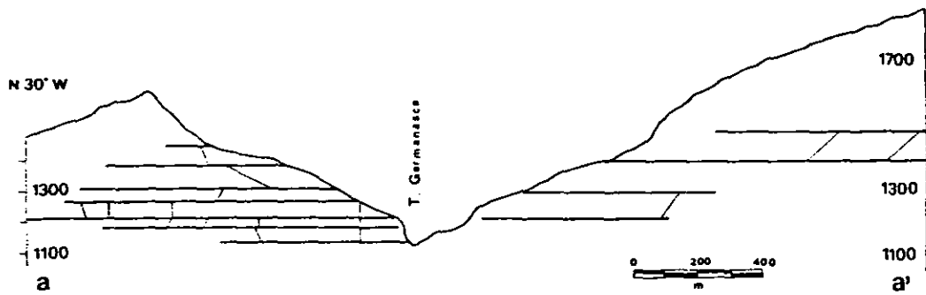
Figure 2. The Fontane talc mine, plan and section, showing the main underground levels.
