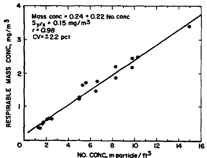
Figure 2. Comparison of dust concentrations obtained from midget impinger and respirable mass dust samples at two perlite processing operations.
