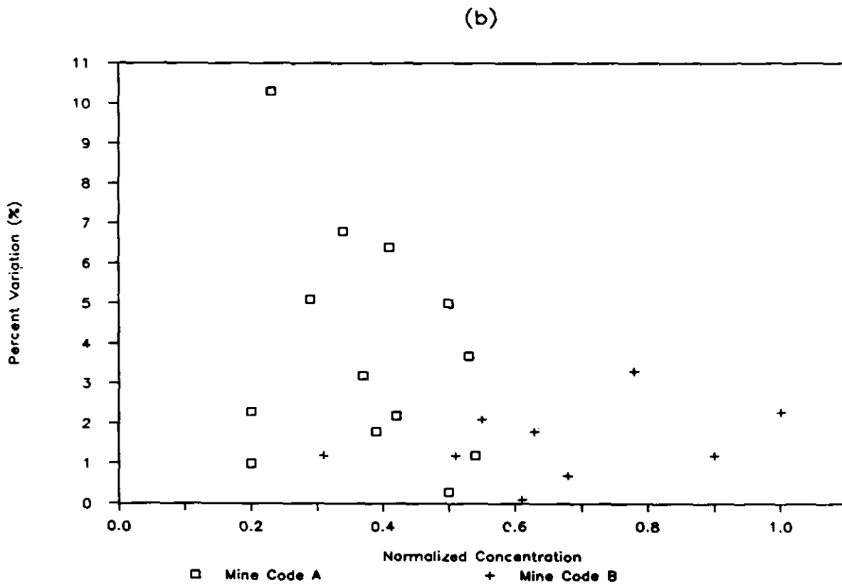
Figure 2. (a) standard deviation and (b) percent variation of concentrations measured at longwalls by Casella Gravimetric Samplers 113A for each field test in Mine A and Mine B.
