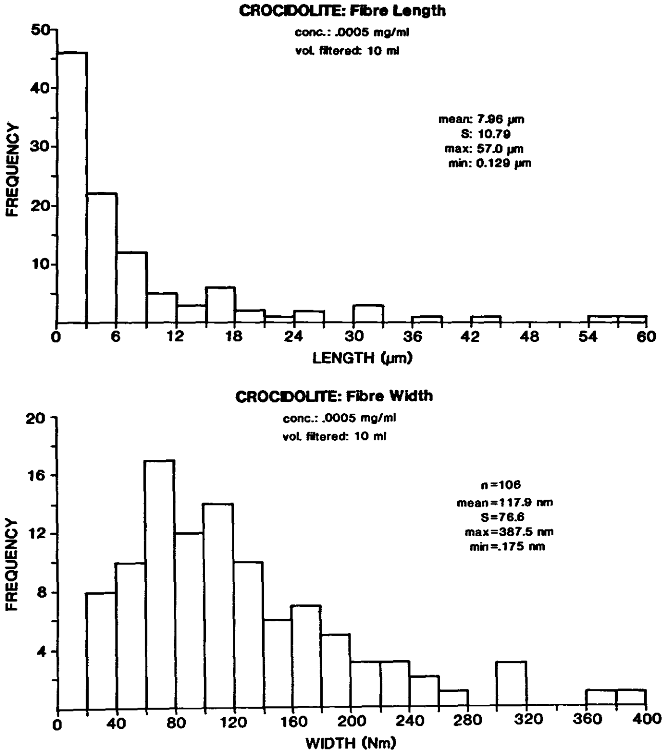
Figure 2. Crocidolite asbestos—fibre dimensions: a) fibre length; b) fibre diameter.
