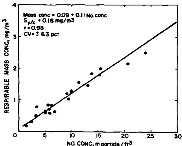
Figure 1. Comparison of dust concentrations obtained from midget impinger and respirable mass dust samples at two graphite processing operations.
