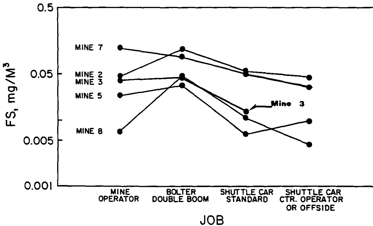
Free Silica Associated with Selected Jobs in Coal Mines, Expressed as Geometric Means (mg/M 3 ).
