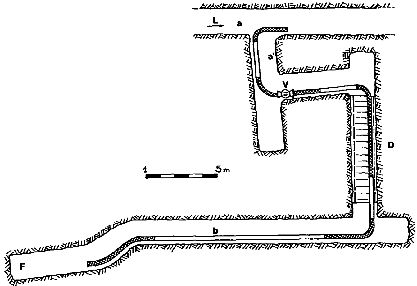
Figure 6. Diagram of stope n.7, Crosetto, where the tests were carried out: L—main level; F—stope face; D—slope; a, a', b, F—sites of measures.
