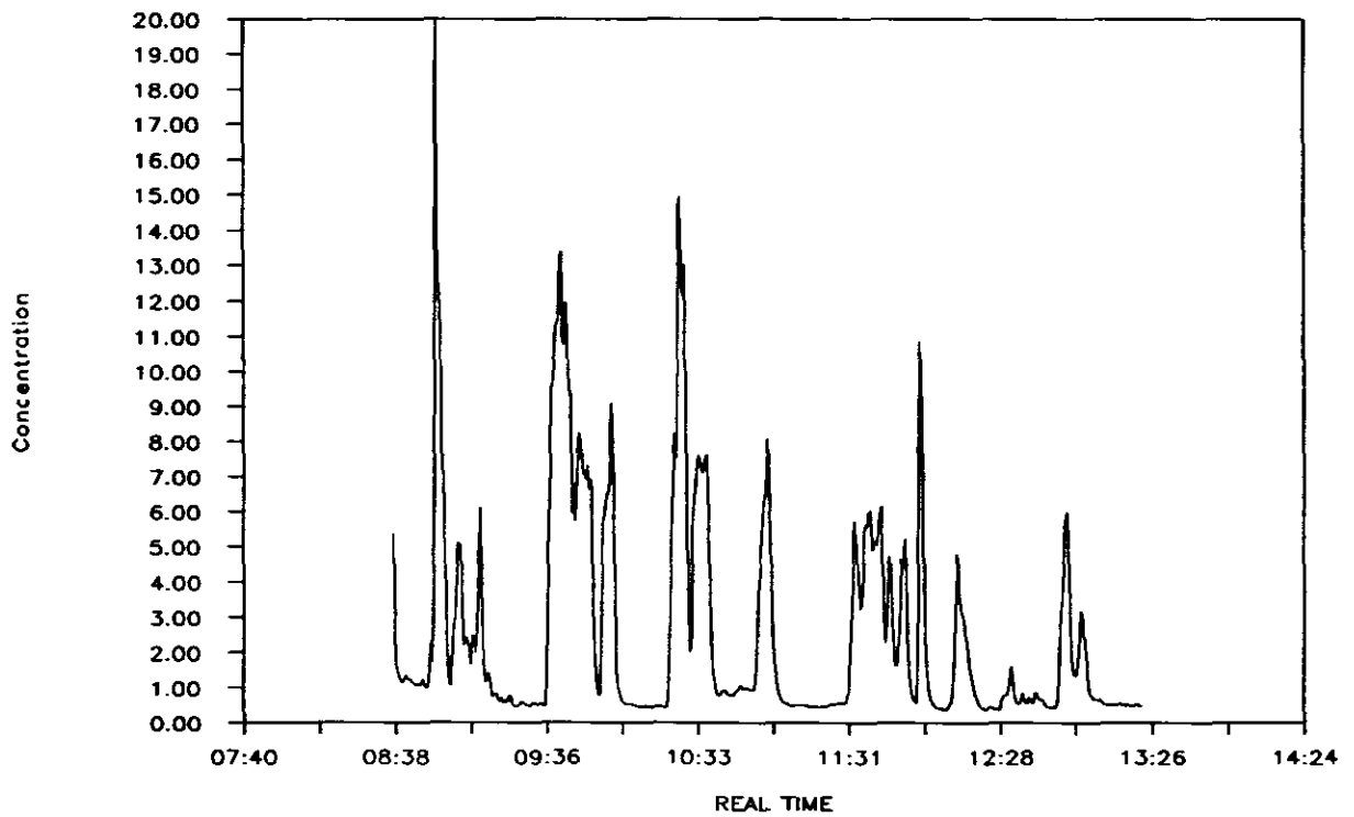
Figure 7. The shift-length concentration recordings (in an arbitrary unit) at the wall section WF of Mine A by (a) SIMSLIN II and by (b) TM-DATA. The time scales of (a) and (b) are in hours and minutes.
