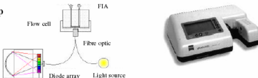
Fig. B.4. Institute for Physical Theoretical Chemistry's compact, low-cost RIS instrument for routine assay measurements.
