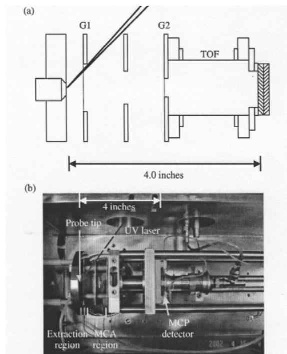
Fig. 5.2. A miniaturized time-of-flight mass spectrometer showing the sample probe, the end cap, and the coaxial detector. (English and Cotter 2003, reprinted with permission).
