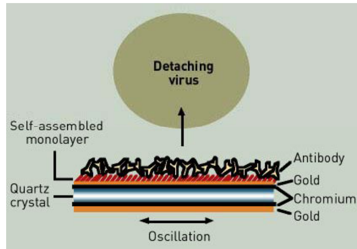
Fig. 6.7. A particle-type-specific piezoelectric biosensor developed at Cambridge University and being commercialized by Akubio, Inc., of Cambridge, UK. A quartz crystal resonator, coated with a receptor, binds an analytical target particle such as a virus. Transverse oscillation of the quartz, induced by applying an alternating voltage across the disc, is deliberately increased in amplitude to the point of bond breakage, releasing acoustic energy that is detected by an external circuit connected to the crystal electrodes. (Adapted from Cooper et al. 2001)
