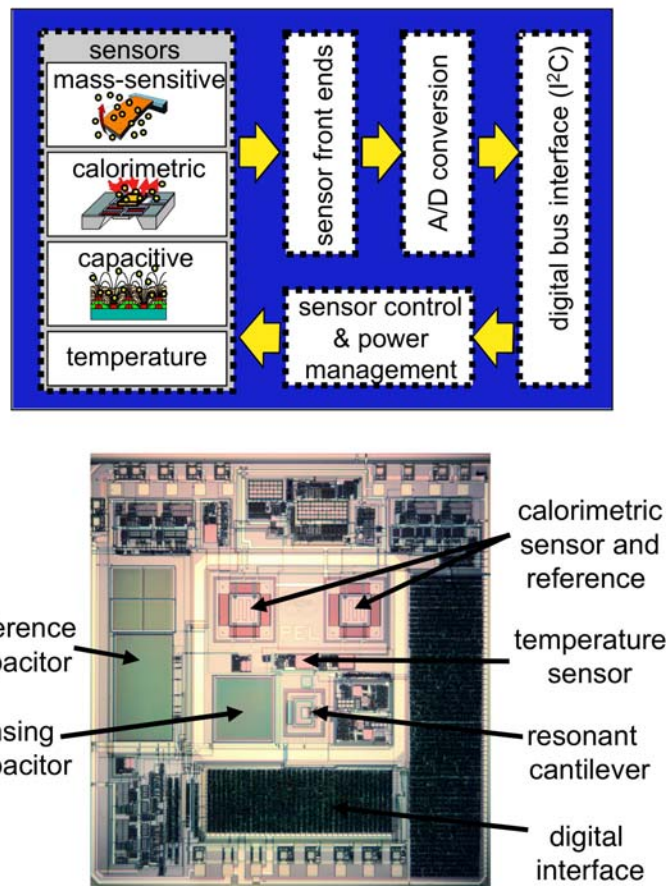
Fig. 6.1. System architecture ( top ) and chip photograph ( bottom ) of an integrated MEMS multisensor combining calorimetric, mass-sensitive, and capacitive sensors to provide chemical discrimination (Hagleitner et al. 2001). In addition to the transducers, this single chip integrates analog-to-digital converters, a digital interface bus, and power management. (Courtesy Dr. A. Hierlemann, Physical Electronics Laboratory, ETH, Zürich)
