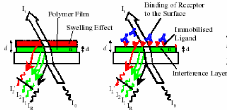
Fig. B.1. Illustration of using principles of reflectometric interference spectroscopy to detect and monitor a wide range of analytes. Left : The transducer element consists of three layers of material, each with different refractive indexes; a shift in the spectrum of the reflected light towards higher wavelengths is directly proportional to the thickness of the top layer. Right : The element contains an immobilized ligand that, when exposed to a protein that binds to it, produces a shifting in the reflected spectrum that is proportional to the amount of protein adsorbed.
