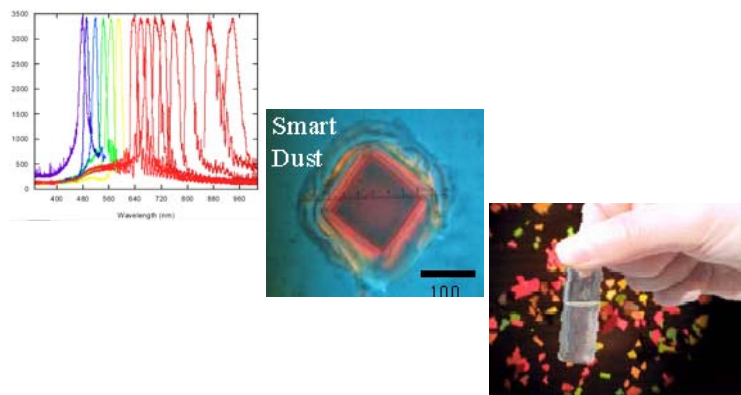
Fig. 2.4. Porous Si particles can be fabricated and used to sense analytes. Left : Spectral properties of different Si particles are due to different interference patterns. Middle : A single particle has nanometer dimensions. Right : A suspension of the Si material dispersed in solvent in a test tube. The background shows an enlargement of the suspension. (Cunin et al. 2002)
