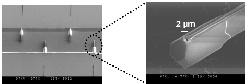
Fig. 6.8. Left : Scanning electron micrograph of a microfluidic channel containing a series of micromachined pipets ( close-up at right ). This is part of a system under development at the University of Twente for the manipulation and analysis of the contents of single living cells. (Courtesy Professor A. van den Berg, University of Twente, The Netherlands)
