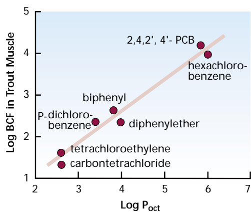
Figure 2.25: Relationship between octanol/water partition ( P_{oct} ) coefficient and bioaccumulation factor (BCF) in trout muscle. Water quality can be inferred by the accumulation of contaminants in fish tissue.
