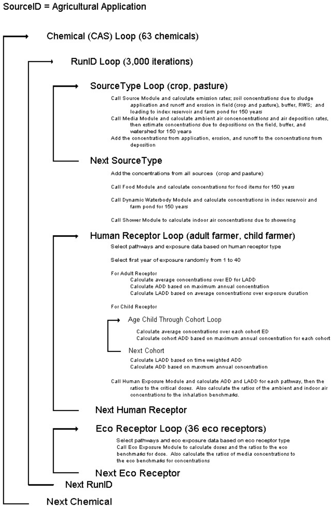
Figure 2-1. Looping structure for agricultural land application modeling.
