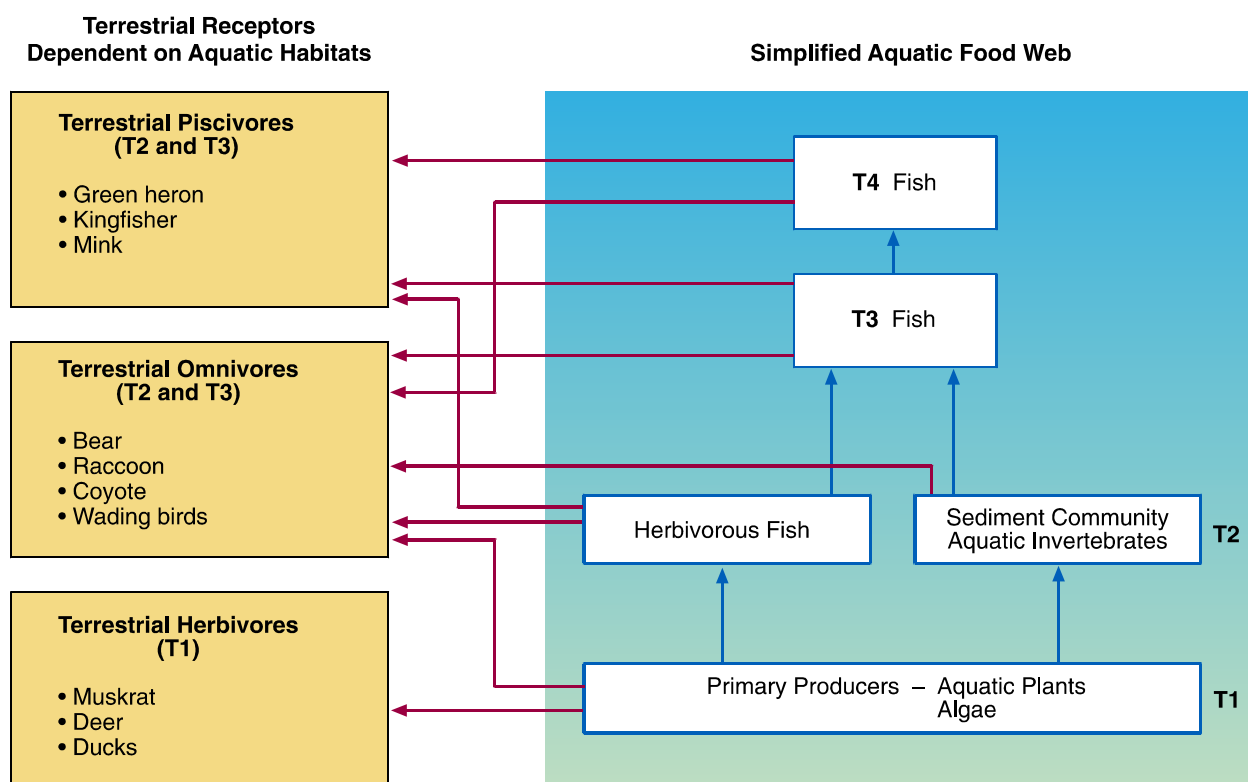
Figure 2-6. Aquatic food web, including example receptors.
