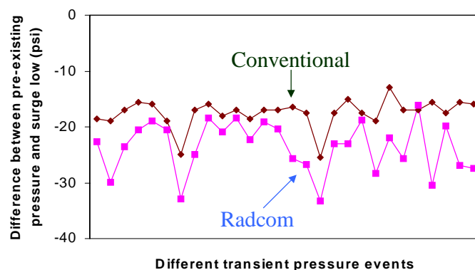
Figure 5. Comparison of the Radcom and Conventional Pressure Recorders for Measurement of Low Pressure Events
