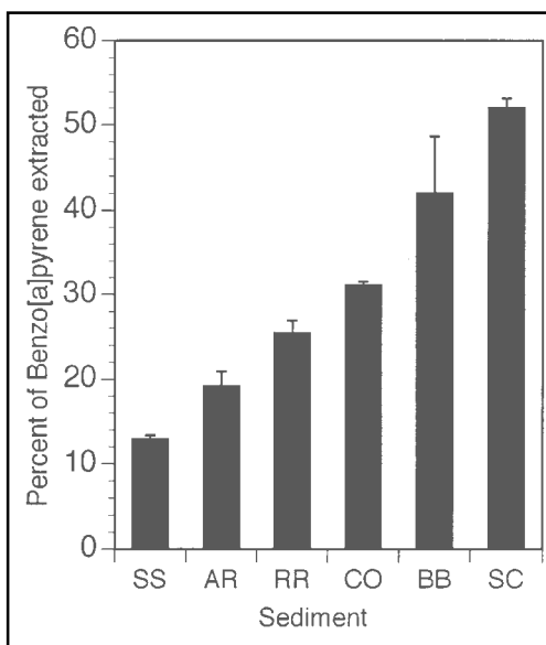
Figure 1. Proportion of sediment-associated benzo[a]pyrene extractable by digestive fluid of Arenicola brasiliensis . Each of the six sediments tested is denoted by a two-letter designation.
