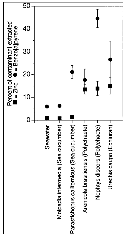
Figure 2. Proportion of zinc and benzo[a]pyrene extractable from a single sediment using the digestive fluids of five invertebrate species. A seawater extraction is shown for comparison.
